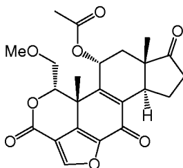
Wortmannin
