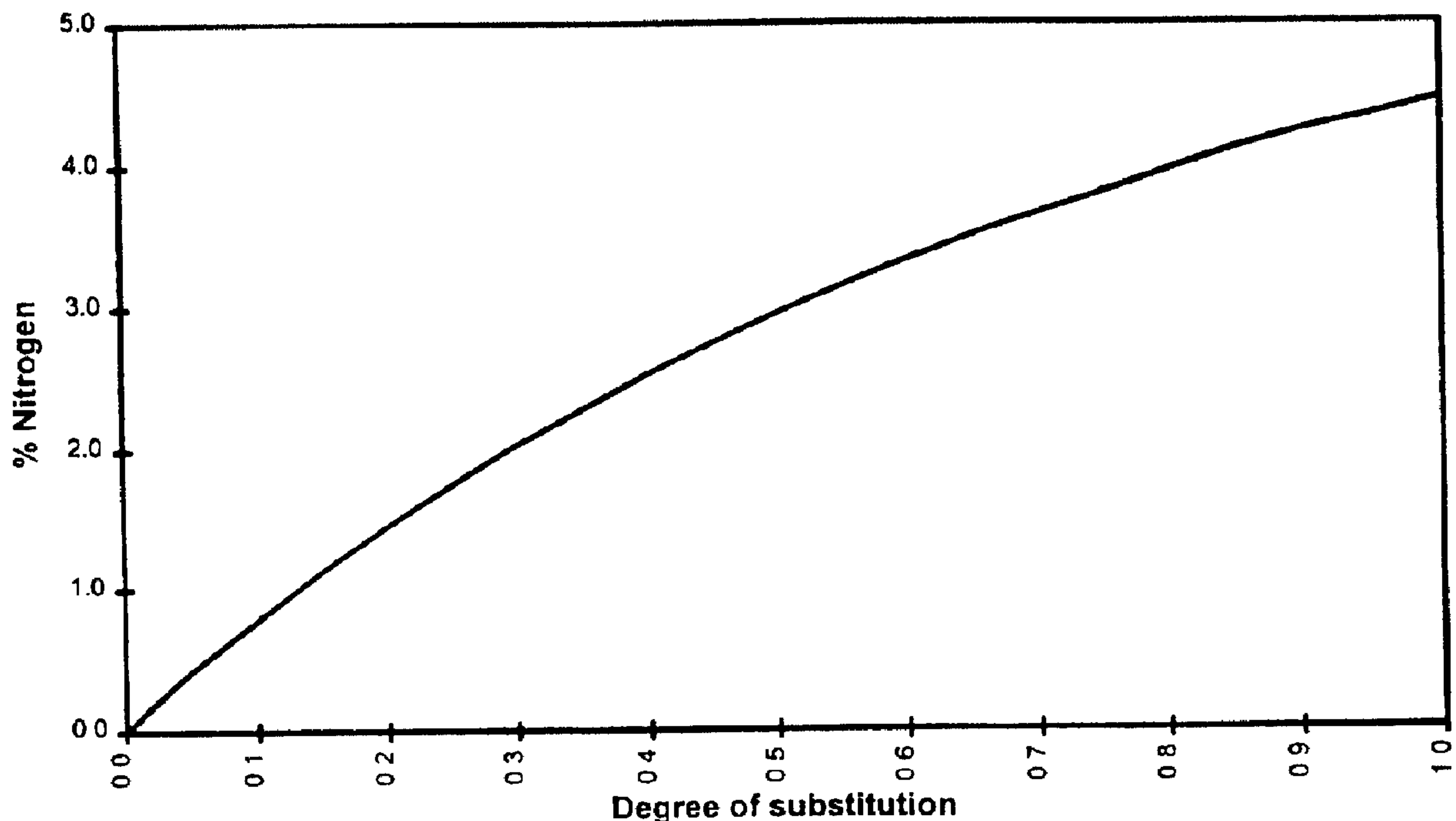
% Nitrogen as a function of degree of substitution for starch cationized using 2,3-epoxypropyl-trimethylammonium chloride.
