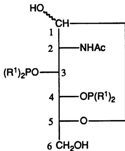
Left-Right diphosphinite from D-Glucose
