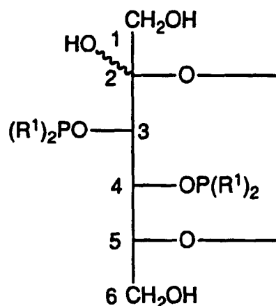
Left-Right diphosphinite from D-Fructose
