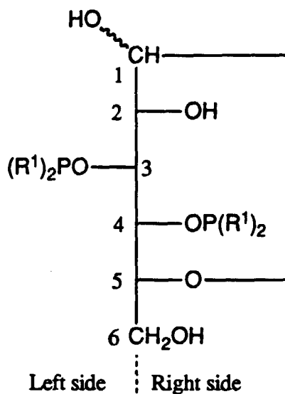
Left-Right diphosphinite from D-Glucose
