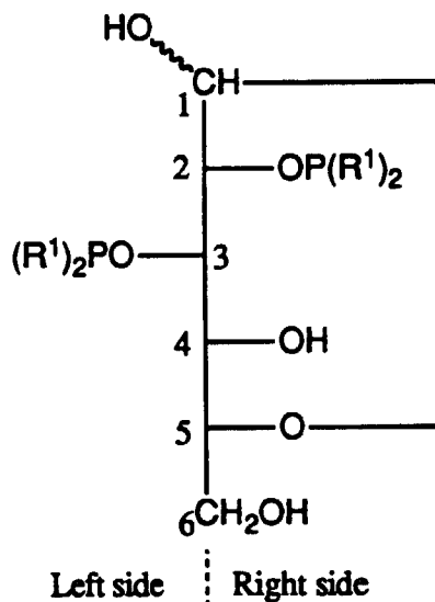
Right-Left diphosphinite from D-Glucose
