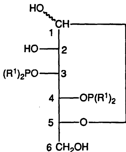
Left-Right diphosphinite from D-Mannose
