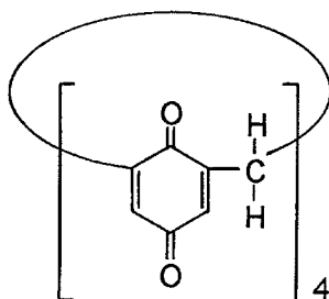
Exemplified Compound (1-1)
