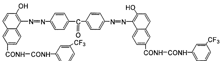
Exemplified Compound (2-1)
