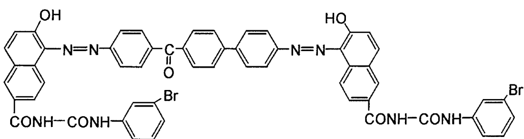
Exemplified Compound (2-12)
