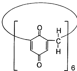
Exemplified Compound (1-2)
