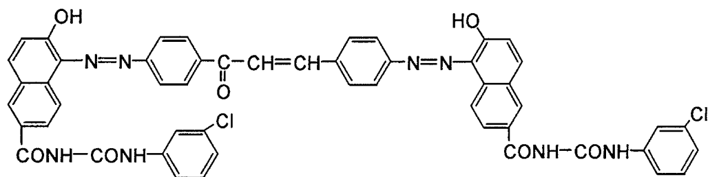
Exemplified Compound (2-10)
