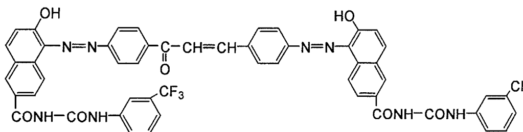
Exemplified Compound (2-11)
