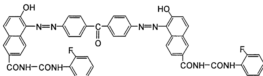
Exemplified Compound (2-3)
