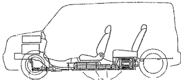
FIG. 3 PRIOR ART
