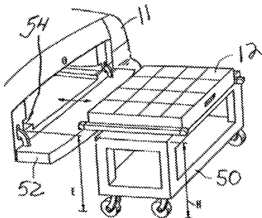
FIG. 5 PRIOR ART
