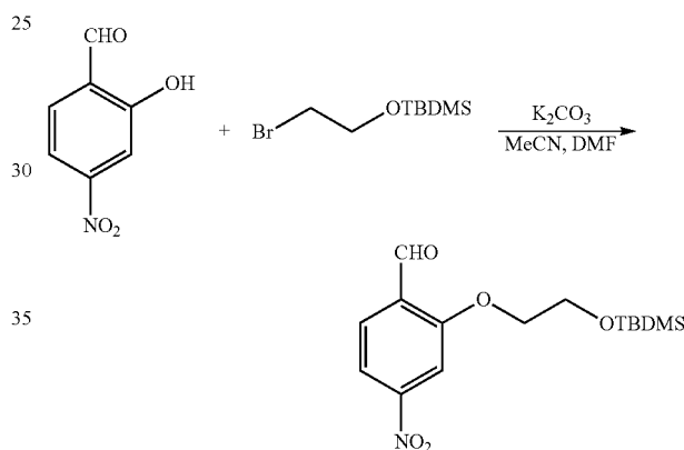
2-([2-tert-Butyldimethylsiloxy]ethoxy)-4-nitrobenzaldehyde
