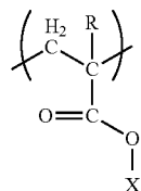
[Chemical Formula 9.]
