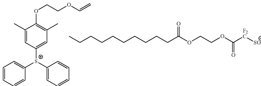
Compound (B1-3)
