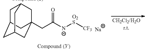
Compound (3')
