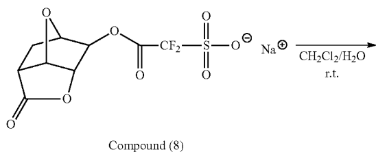
Compound (8)
