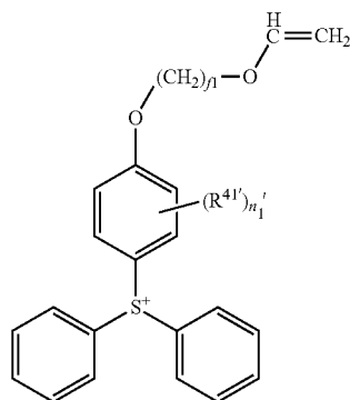
[Chemical Formula 34.]
