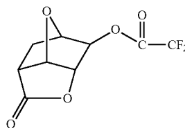
Compound (8)
