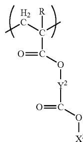
[Chemical Formula 10.]
