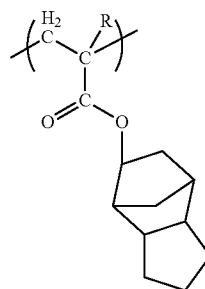
[Chemical Formula 31.]
