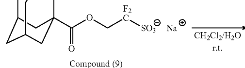
Compound (9)
