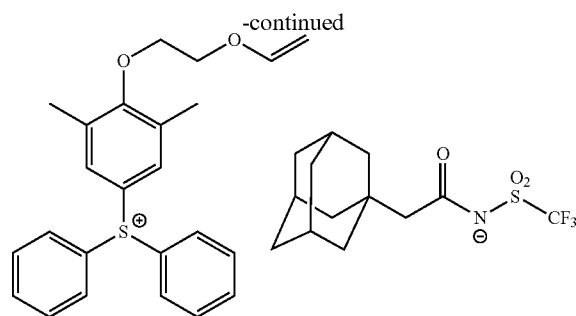
Compound (B1-1')
