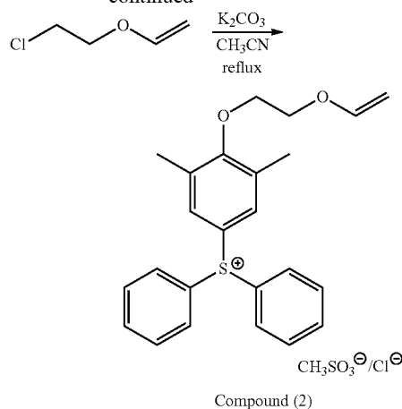
Compound (2)
