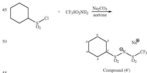
Compound (4')
