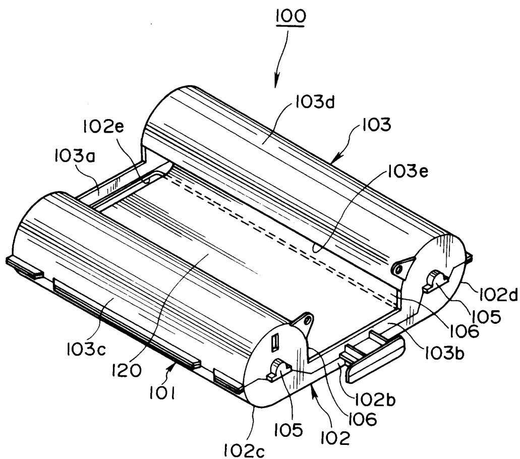
FIG.13 (PRIOR ART)
