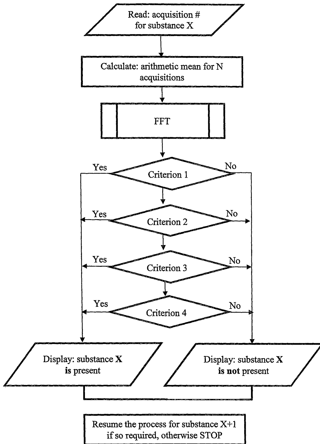
Figure 4. Workflow of the method for detecting potentially explosive substances, explosives and drugs
