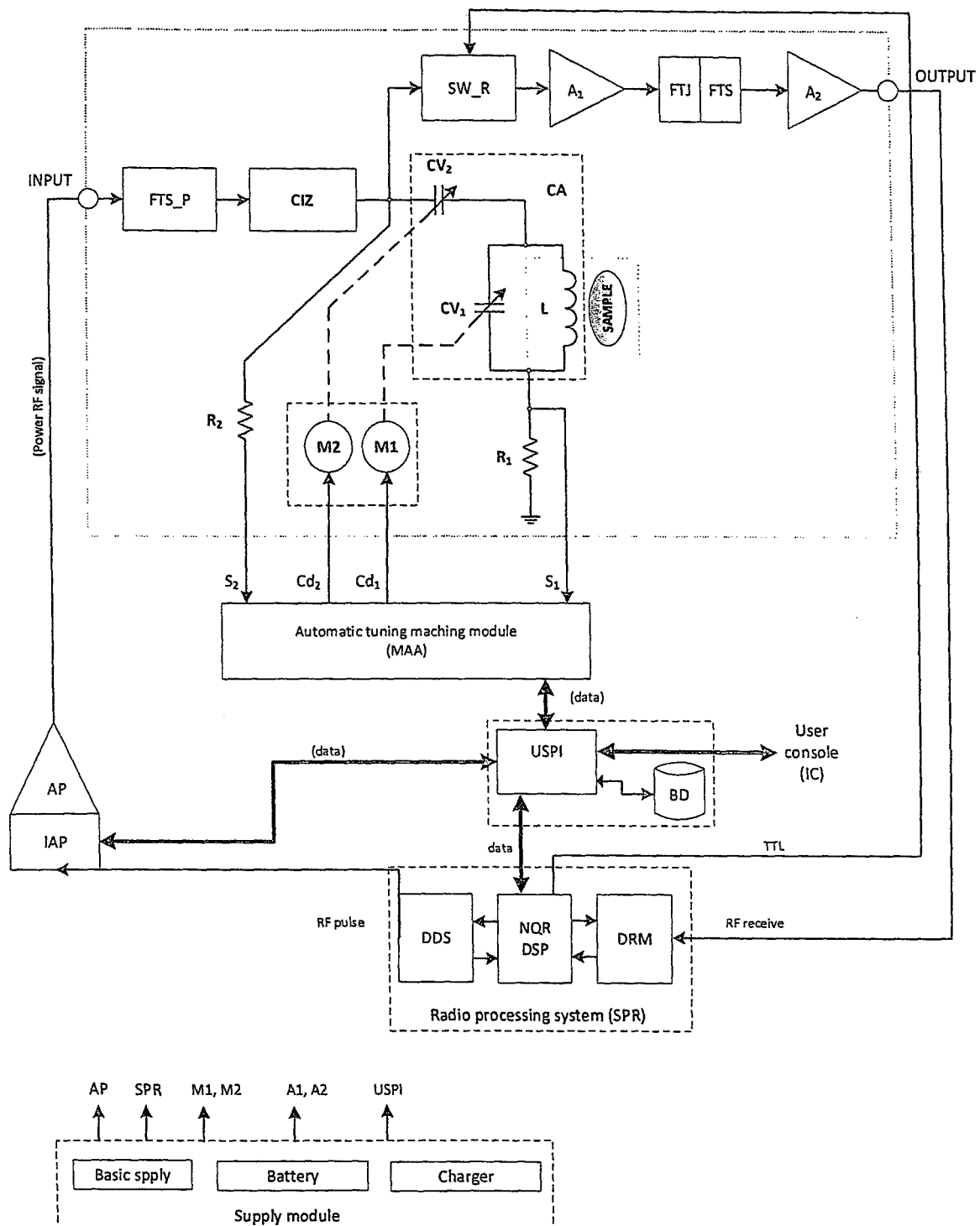
Figure 3. Block diagram of the mobile detector (the central processing unit - UC)
