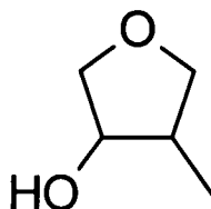
3-Furanol, tetrahydro-4-methyl-
