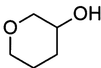
Tetrahydropyran-3-ol
