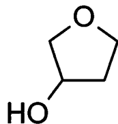
Tetrahydrofuran-3-ol
