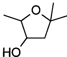
3-Furanol, tetrahydro-2,5,5-trimethyl-
