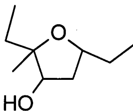
3-Furanol, Tetrahydro-2, 5-Diethyl-2-Methyl-
