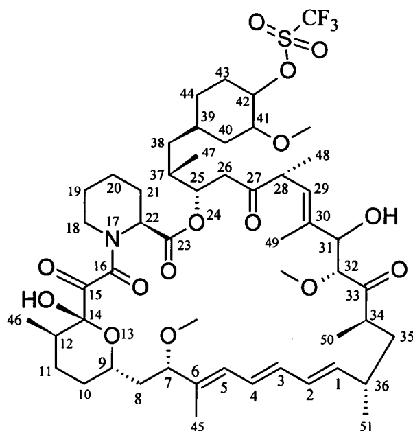
42-O-(trifluoromethylsulfonyl) rapamycin
