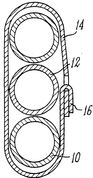
FIG. 2 PRIOR ART
