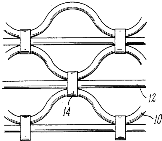
FIG. 1 PRIOR ART
