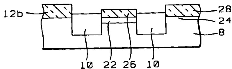
FIG. 2c - Prior Art
