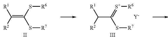
Reaction scheme 1:
