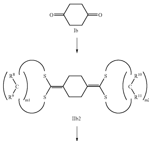
Reaction scheme 4
