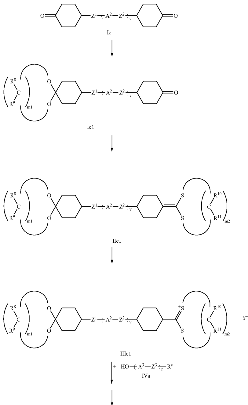
Reaction scheme 7
