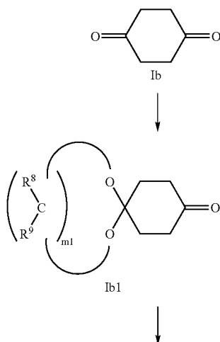
Reaction scheme 6
