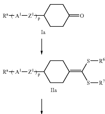
Reaction scheme 2
