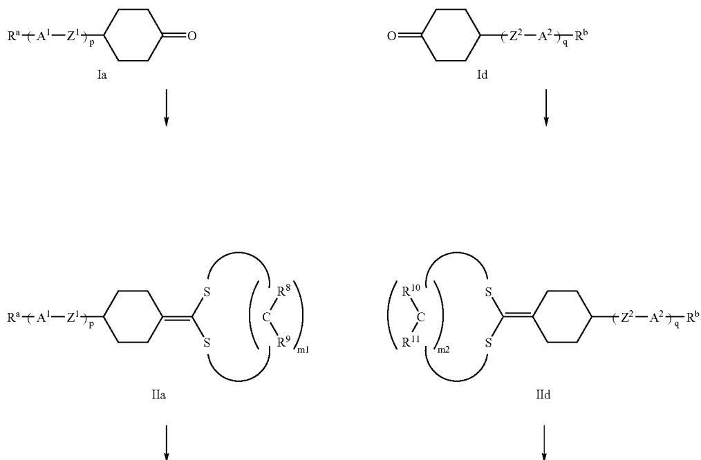
Reaction scheme 3
