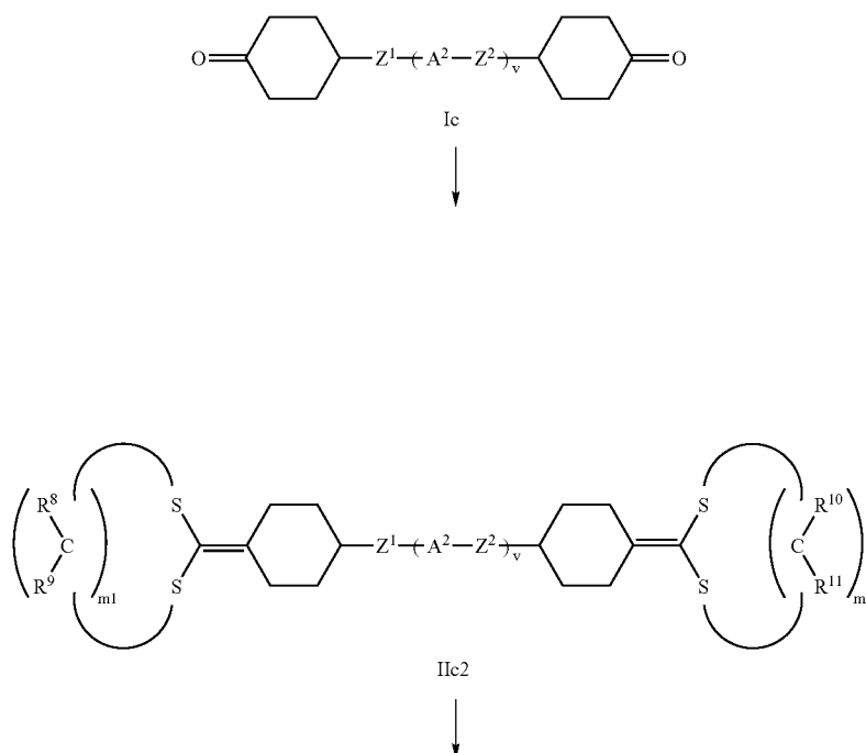
Reaction scheme 5
