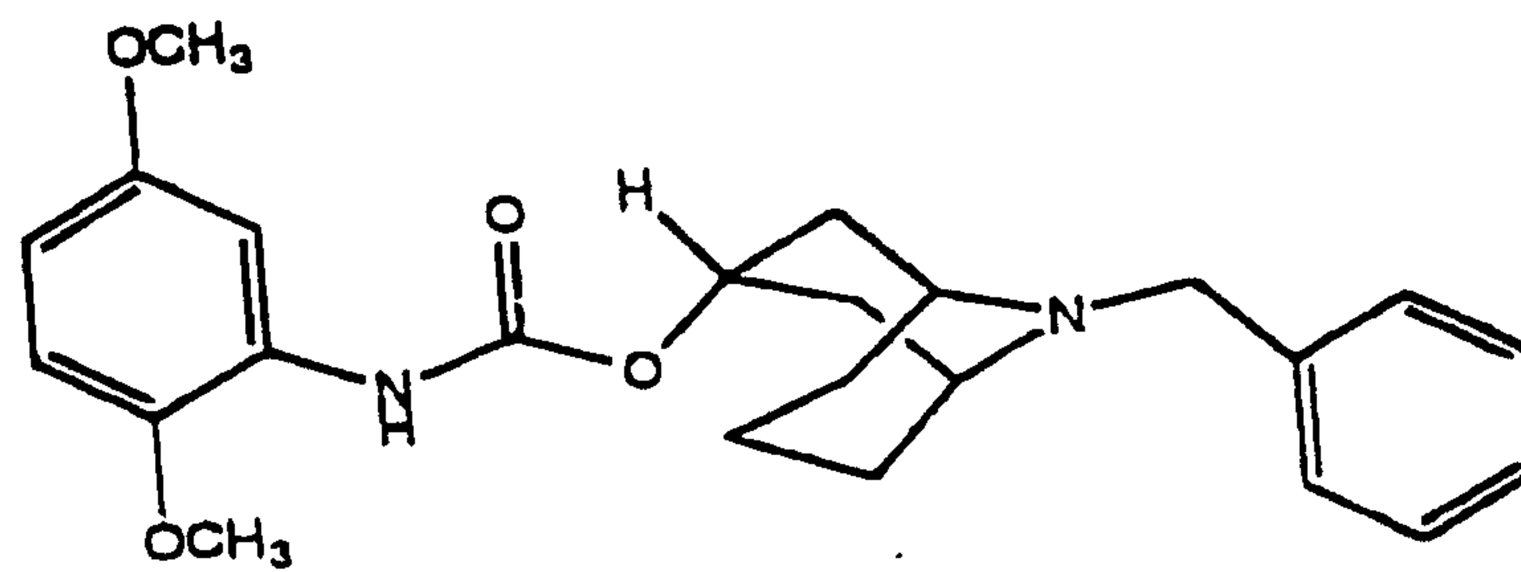
Compound 5
