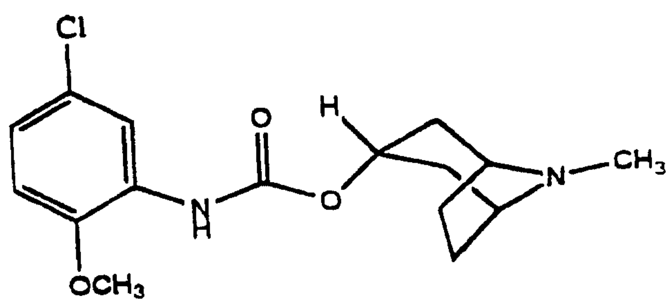
Compound 3
