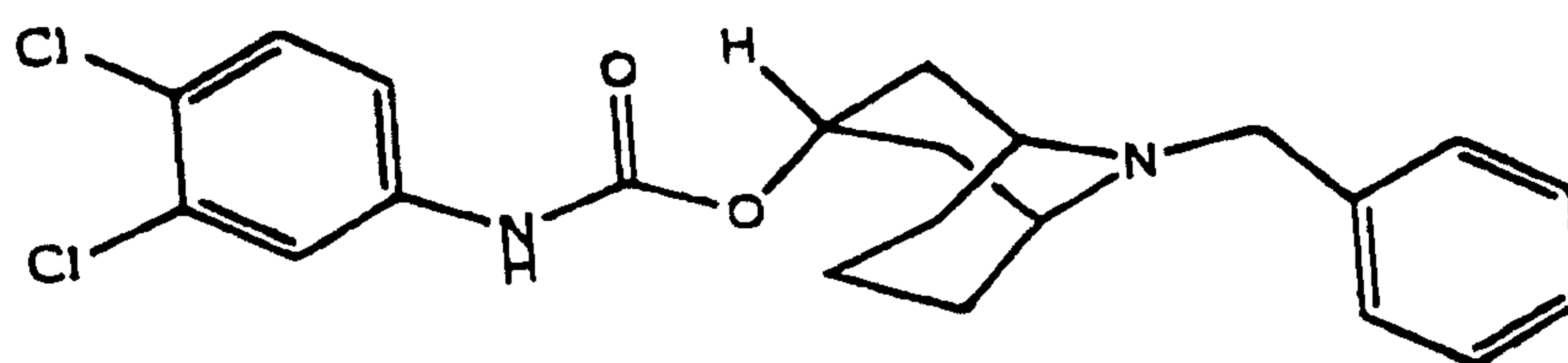
Compound 4
