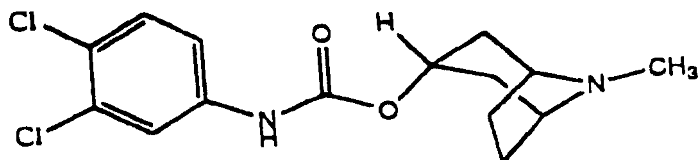
Compound 2
