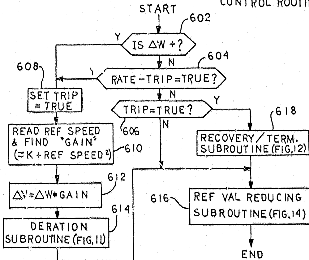
FIG. 10 WHEELSLIP MODE CONTROL ROUTINE
