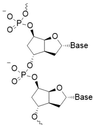
Structure of 7'-5'-alpha-anomeric-bicyclo-DNA
