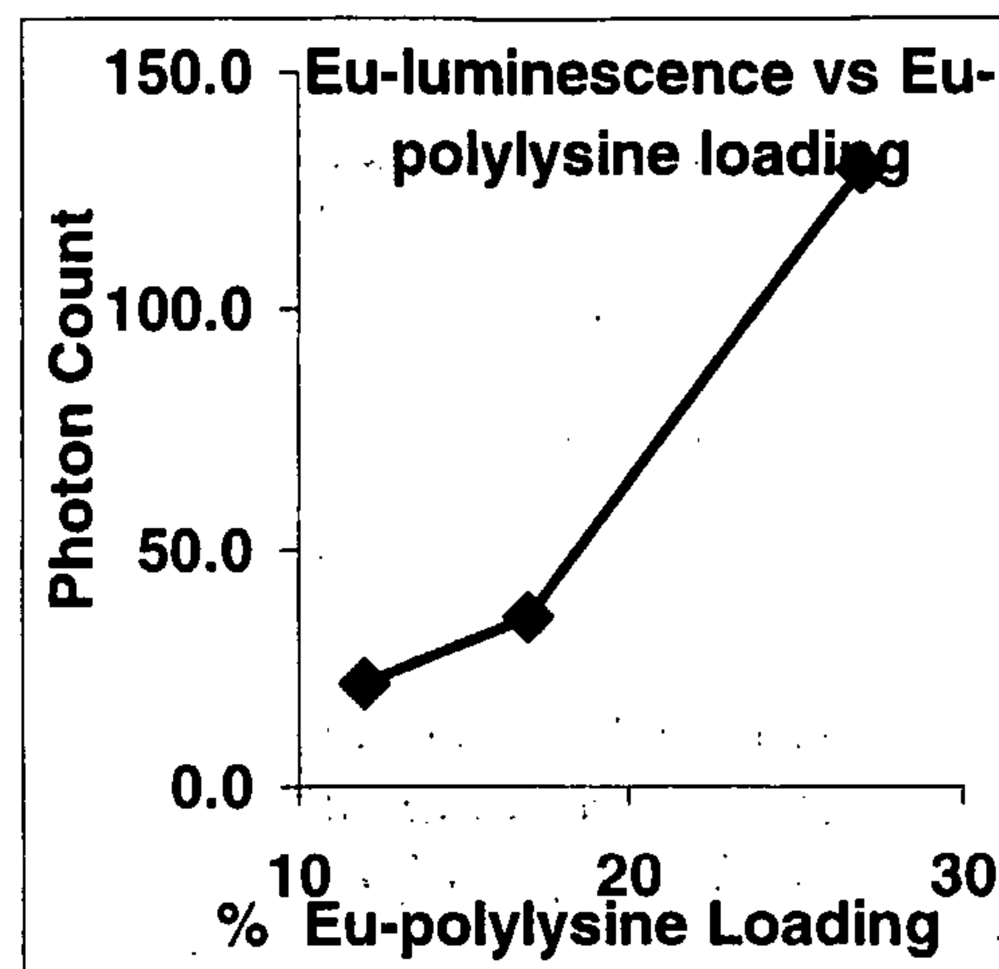
Figure 2. Eu(III) emission at 618 nm normalized to 1 \times 10^{-6} mmol polylysine /mL, as a function of Eu-polylysine percentage loading.
