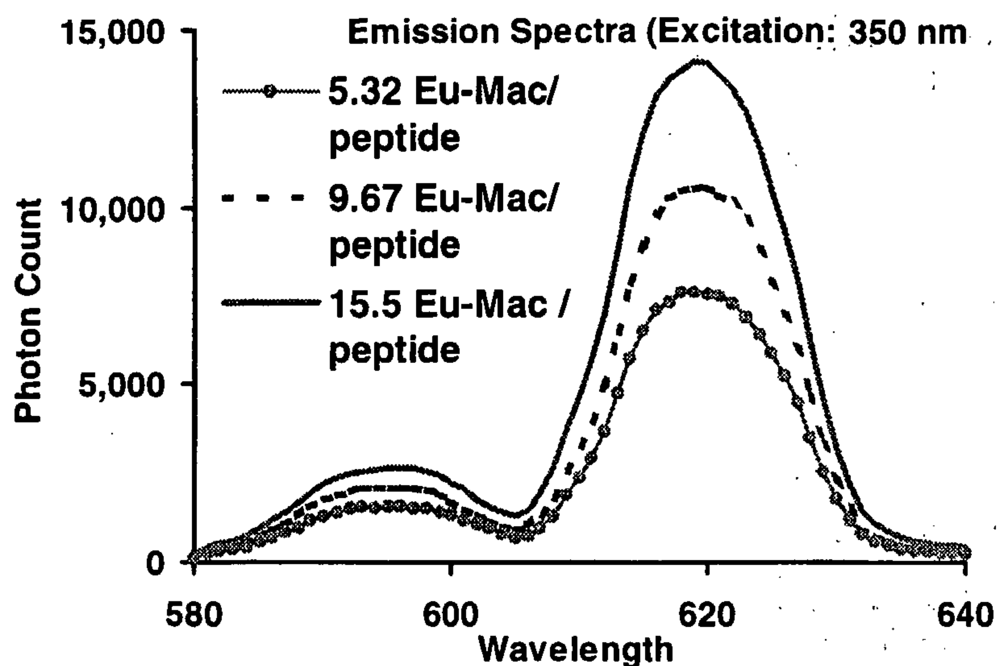
Figure 4. Eu-Emission spectra of EuMac-Polylysine-phenylalanine conjugates as a function of different Eu MacNCS/polylysine-phenylalanine ratios used in the coupling reactions.
