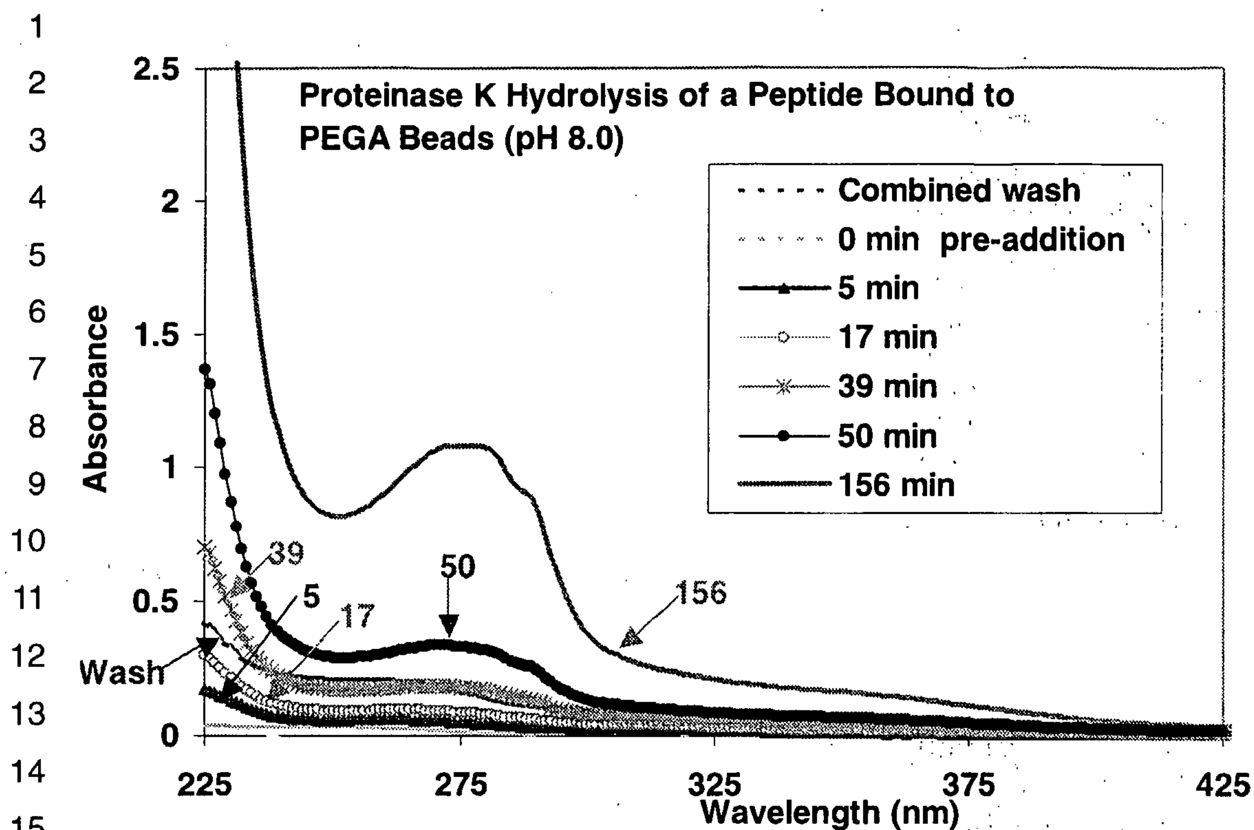
Figure 9. Proteinase K (14.2ug/mL) hydrolysis at pH 8.01 of the Peptide-PEGA-Beads (1.1mg). The spectra indicate that with time (5 to 156 min), Proteinase K cleaves the peptide, and that the released peptide includes both tryptophan and NpyS. A small amount of the Peptide bound to the Peptide-PEGA-Beads is initially washed off (Combined Wash). The preaddition, 0-min sample shows minimal background. At pH 8 the NpyS absorbance at 350nm is reduced.
