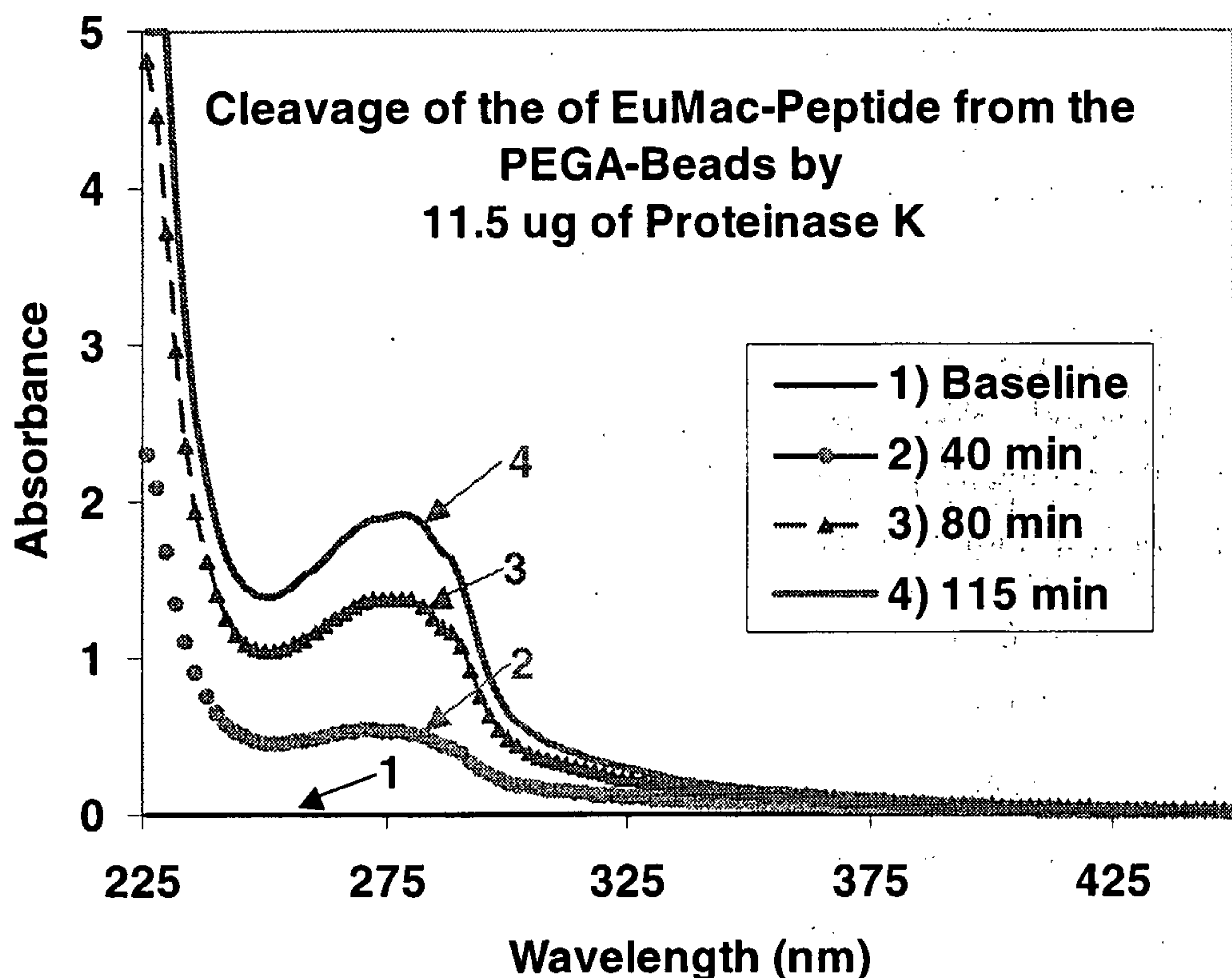
Figure 12. Graph of supernatant from Proteinase K hydrolysis of EuMac-(mono)-NCS and NIRL-2 beads conjugate. The graph shows that the absorbance at about 280 nm increases with time for all samples. The longer the hydrolysis time, the higher the absorbance results at about 280 nm. This demonstrates that Proteinase K cleaves the peptide from the PEGA-Beads.
