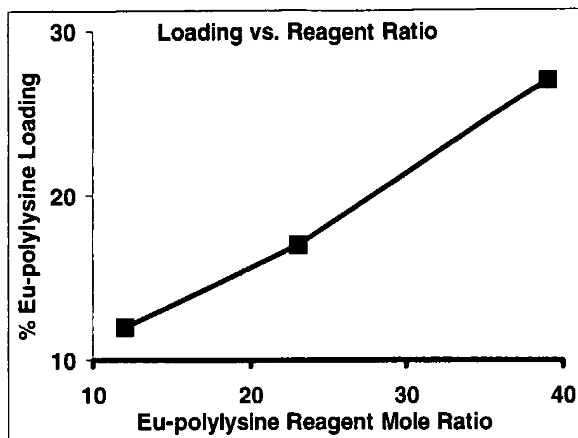
Figure 1. Plot of the average EuMac-to-polylysine loading in coupled polylysine versus the EuMac-di-NCS-to-polylysine mole ratio used in the coupling reaction. The loading is expressed as percentage of EuMac-coupled lysine residues.
