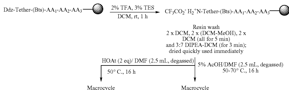
Scheme 2: Alternative Cyclization Methodologies
