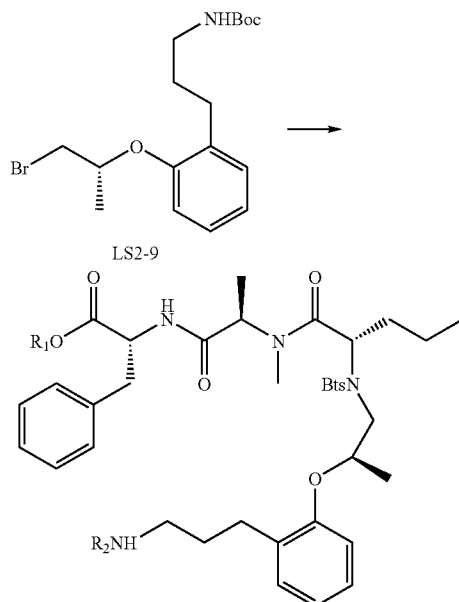
LS2-25 ( R_1 = t\text{Bu} , R_2 = \text{Boc} ) LS2-23 ( R_1 = R_2 = \text{H} )
