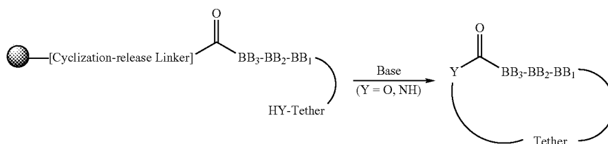
Scheme 1: Cyclization-release Strategy
