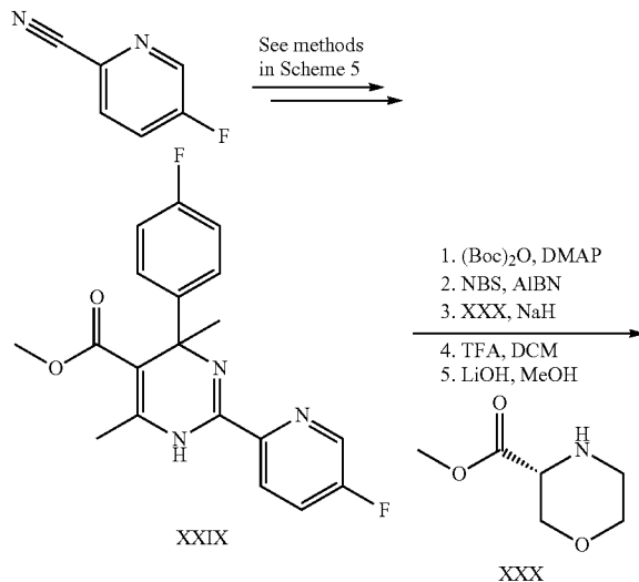
Scheme 8
