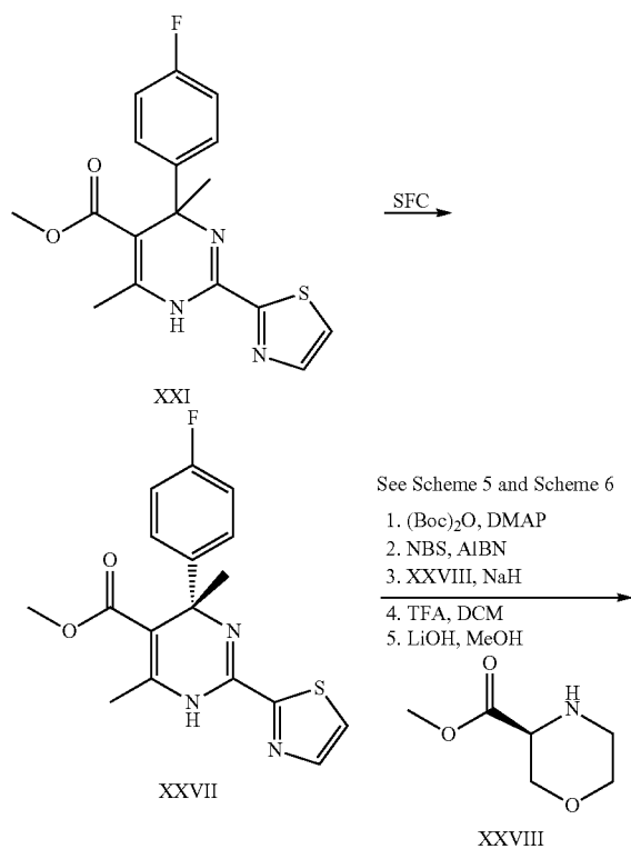
Scheme 7
