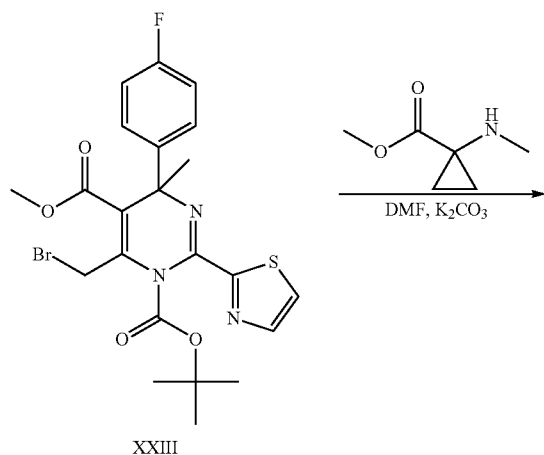
Scheme 6
