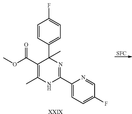
Scheme 11
