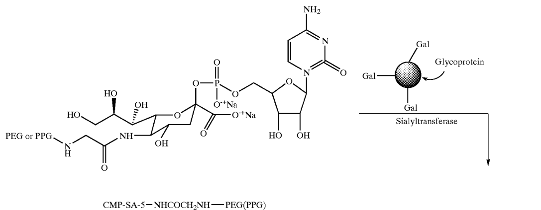
Scheme 12
