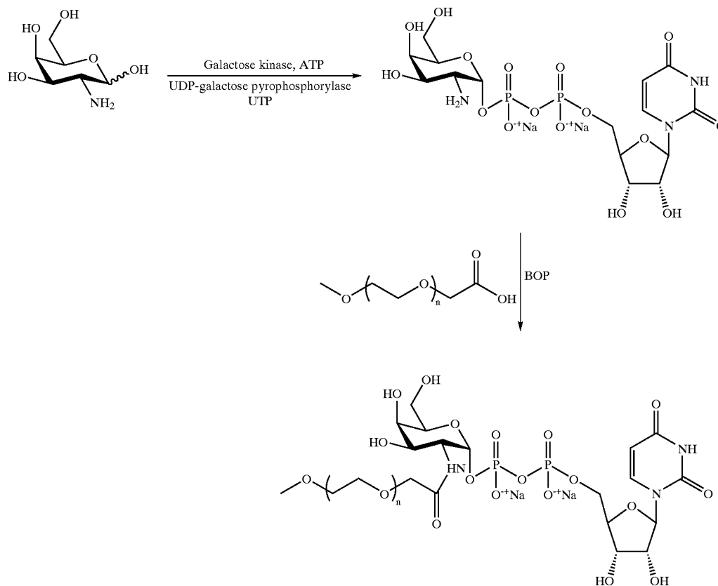
Scheme 11
