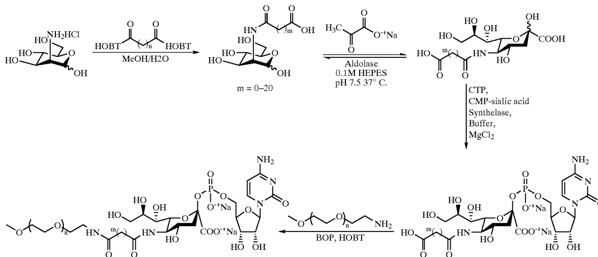
Scheme 6
