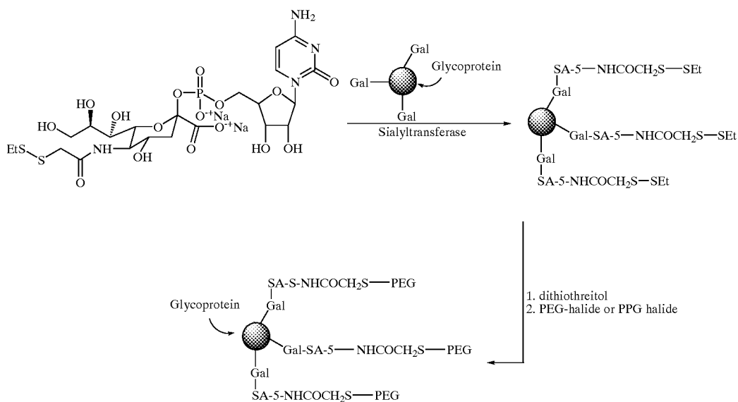
Scheme 13
