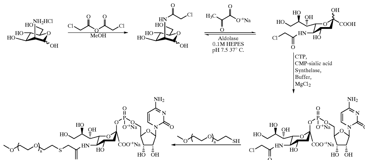
Scheme 5
