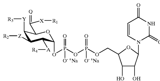
UDP-galactose-derivatives
