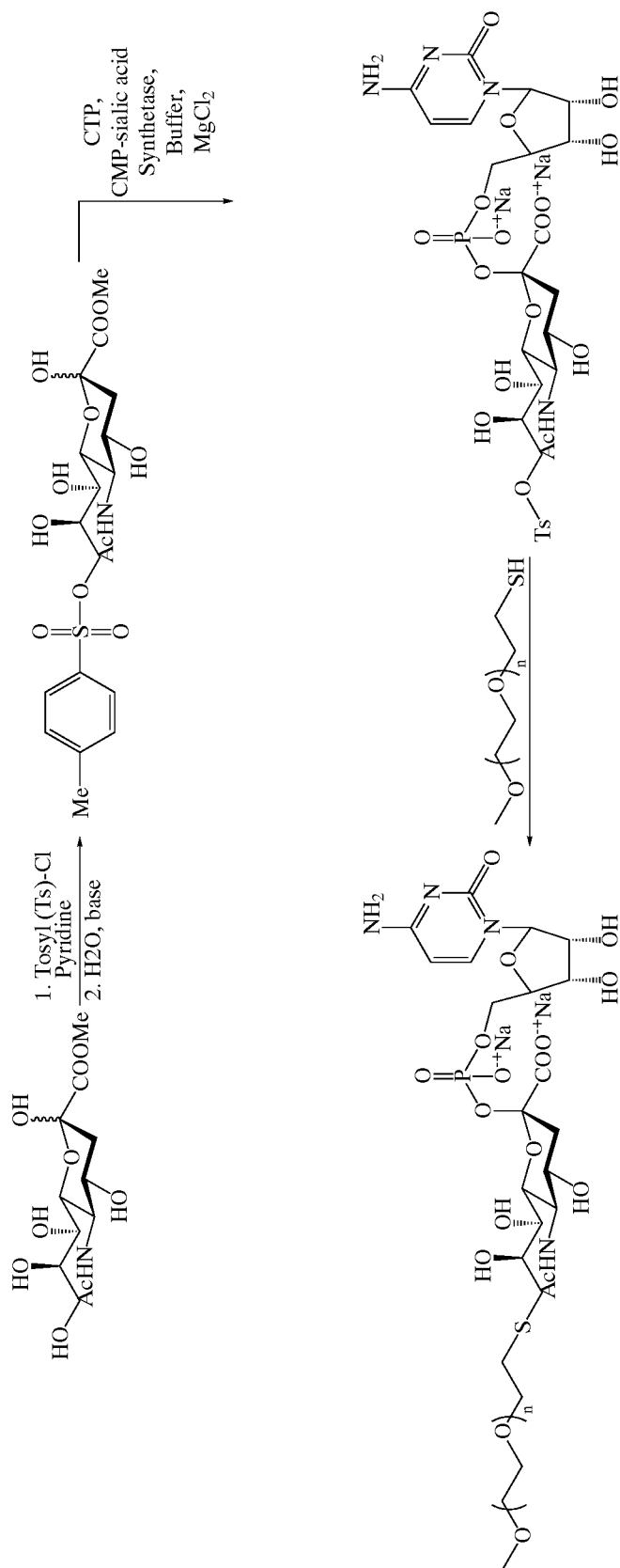
Scheme 7
