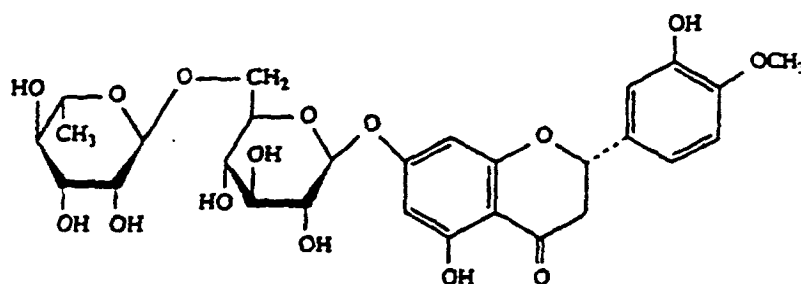
Hesperidin
