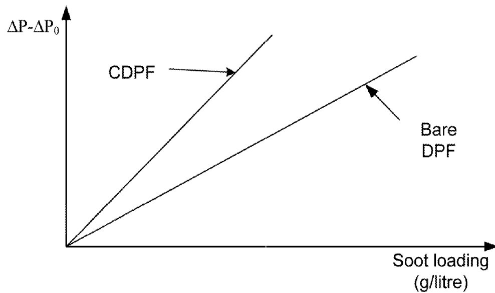
Figure 6 - Modified pressure drop versus soot loading in practice
