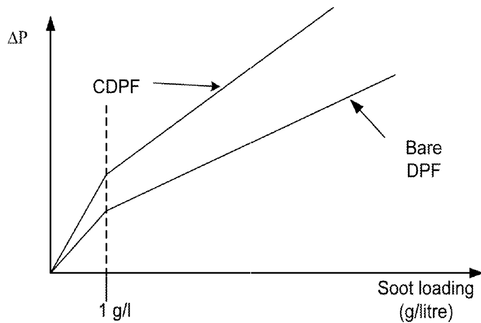
Figure 5 - Pressure drop versus soot loading
