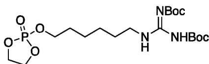
phosphoester based monomer
