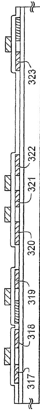
FIG. 4A STEP OF ADDING N-TYPE IMPURITY ELEMENT
