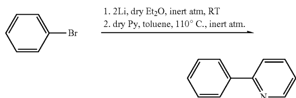
Scheme 5: Synthesis of 2-phenylpyridine.
