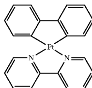
(Biphenylinato-C,C)- (bipyridinato-N,N) Pt(II) Pt(bph)(bpy)(4)
