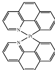
cis-Bis[benzo(h) quinolinato-N,C] Pt(II) Pt(Bhq) 2 (3)
