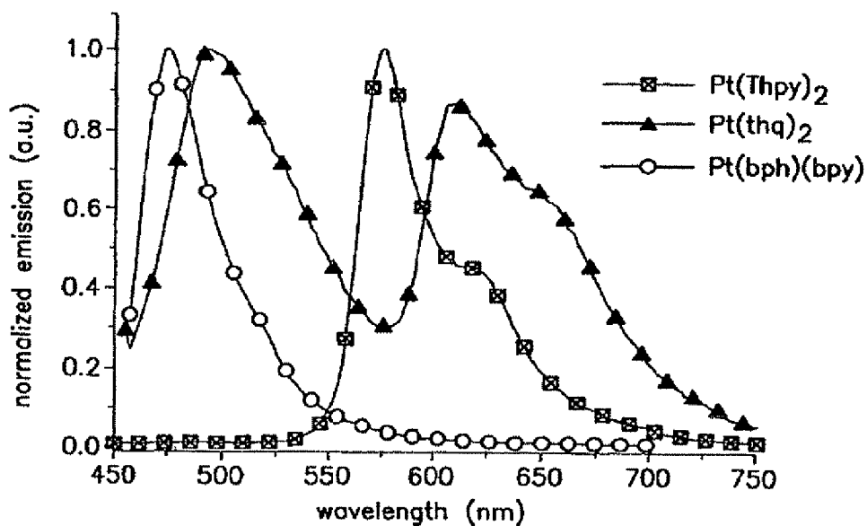
Emission spectra of the complexes.
