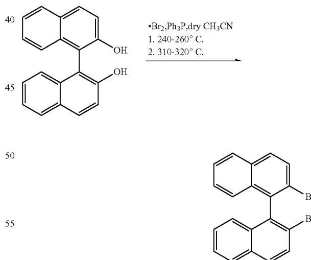
Scheme 7: Synthesis of 2,2'-dibromo-1,1'-binaphthyl.
