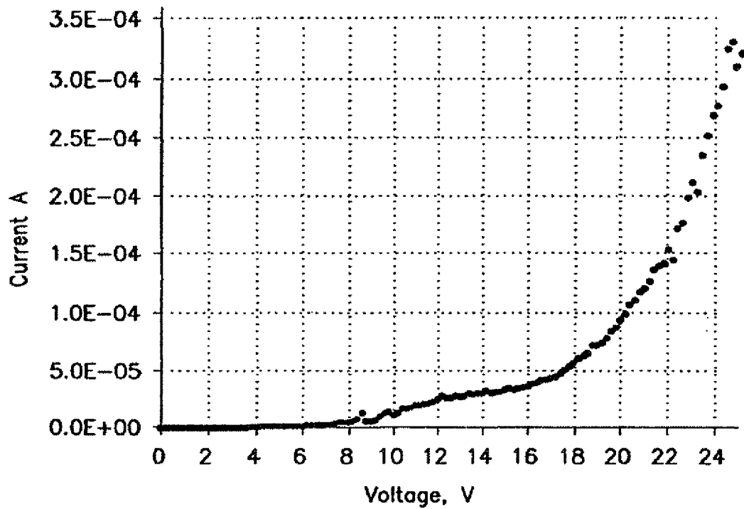
I-V characteristic of the device.
