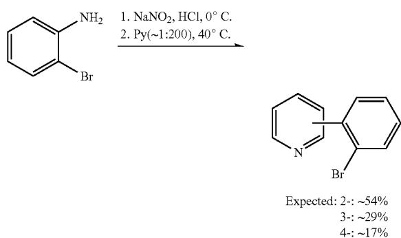
Scheme 4: Synthesis of n-(2'-bromophenyl)pyridines.
