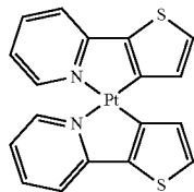
cis-Bis[2-(2'-thienyl) pyridinato-N,C 3 ] Pt(II) Pt(Thpy) 2 (2)
