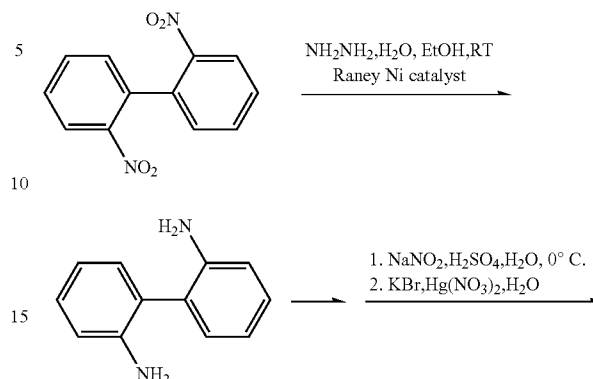
Scheme 6: Synthesis of 2,2'-dibromobiphenyl from 2,2'-dinitrobiphenyl.
