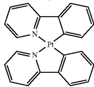
cis-Bis[2-(2-phenyl) pyridinato-N,C 2 ] Pt(II) Pt(Phpy) 2 (1)
