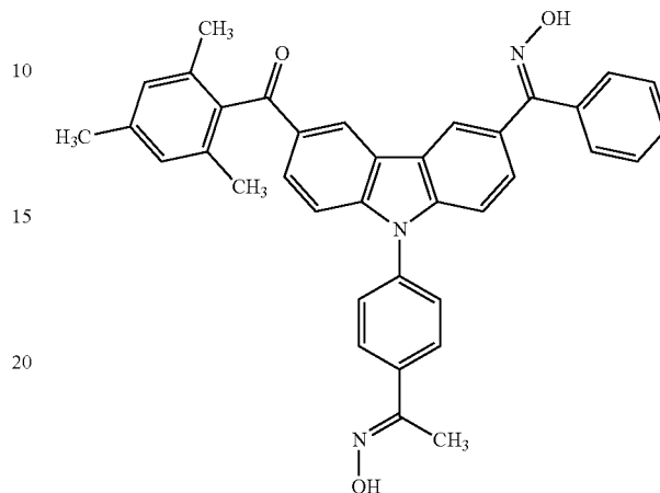
12.c [9-[4-[N-hydroxy-C-methyl-carbonimidoyl]phenyl]-6-[N-hydroxy-C-phenyl-carbonimidoyl]carbazol-3-yl]-(2,4,6-trimethylphenyl)methanone
