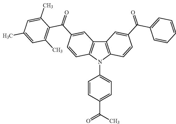
12.b 1-[4-[3-benzoyl-6-(2,4,6-trimethylbenzoyl)carbazol-9-yl]phenyl]ethanone
