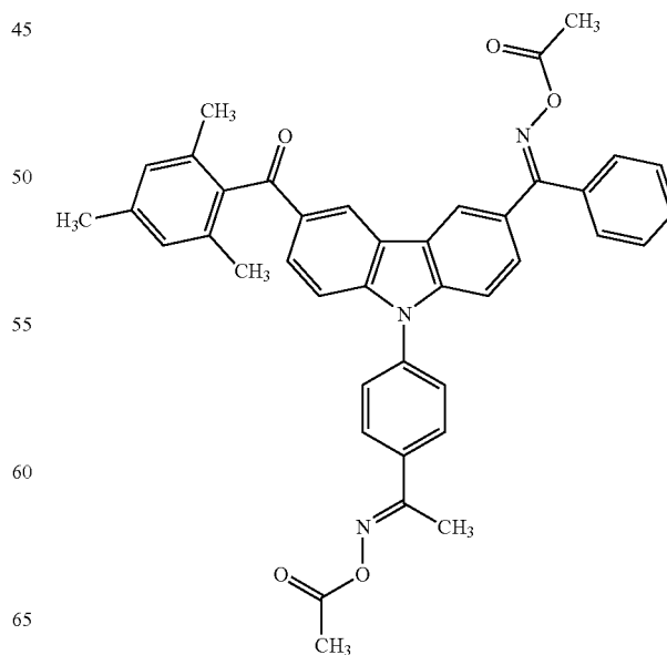
12.d [1-[4-[3-[N-acetoxy-C-phenyl-carbonimidoyl]-6-(2,4,6-trimethylbenzoyl)carbazol-9-yl]phenyl]ethylideneamino] acetate
