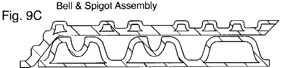
PRIOR ART
