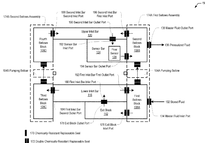
Fluid Flow Using Double Seals Block Diagram
