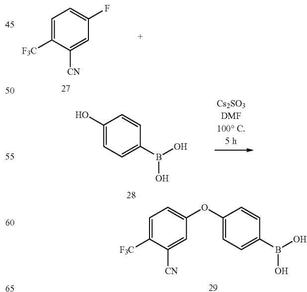
Scheme 18
