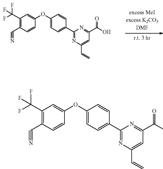
Scheme 8
