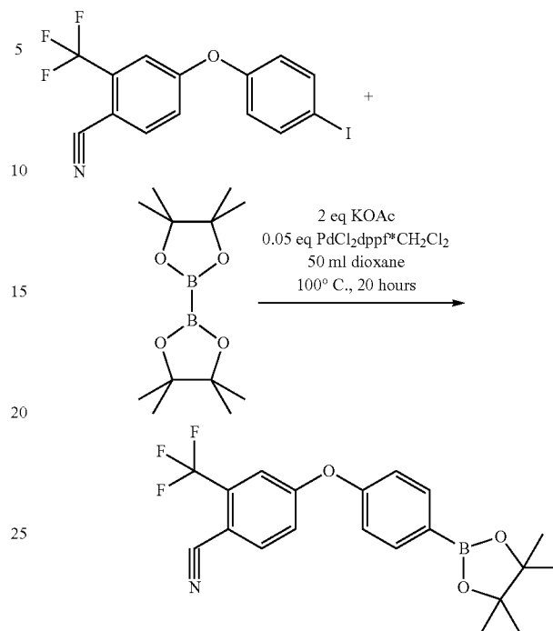
Scheme 6
