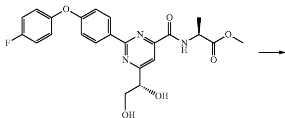
Scheme 17
