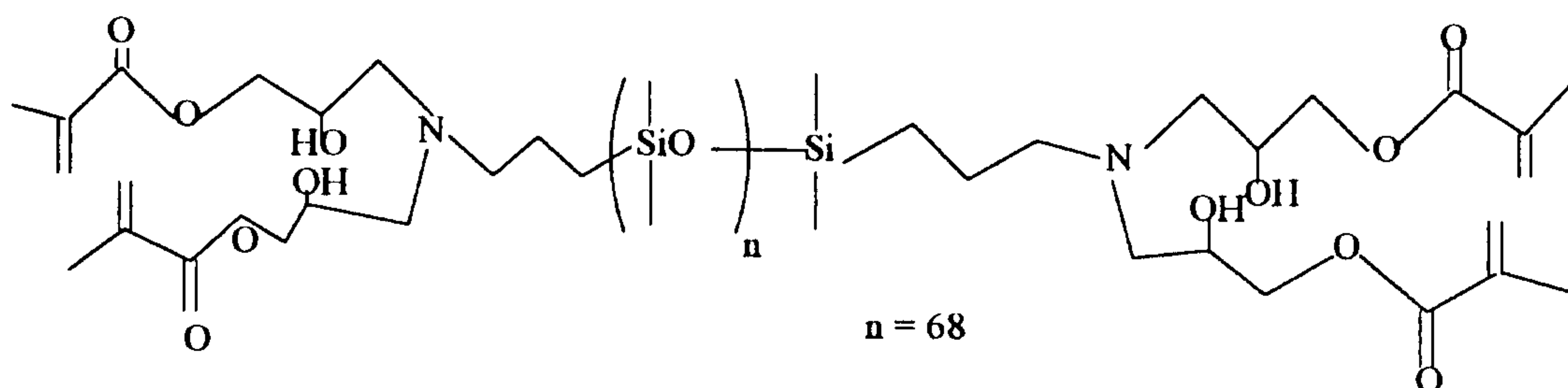
Structure V.
