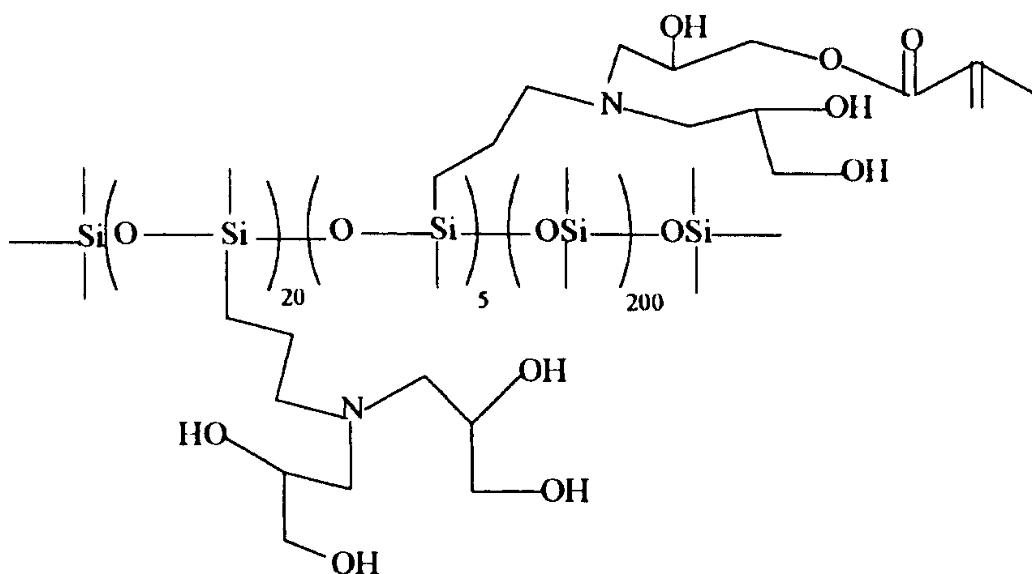
Structure VIII,
