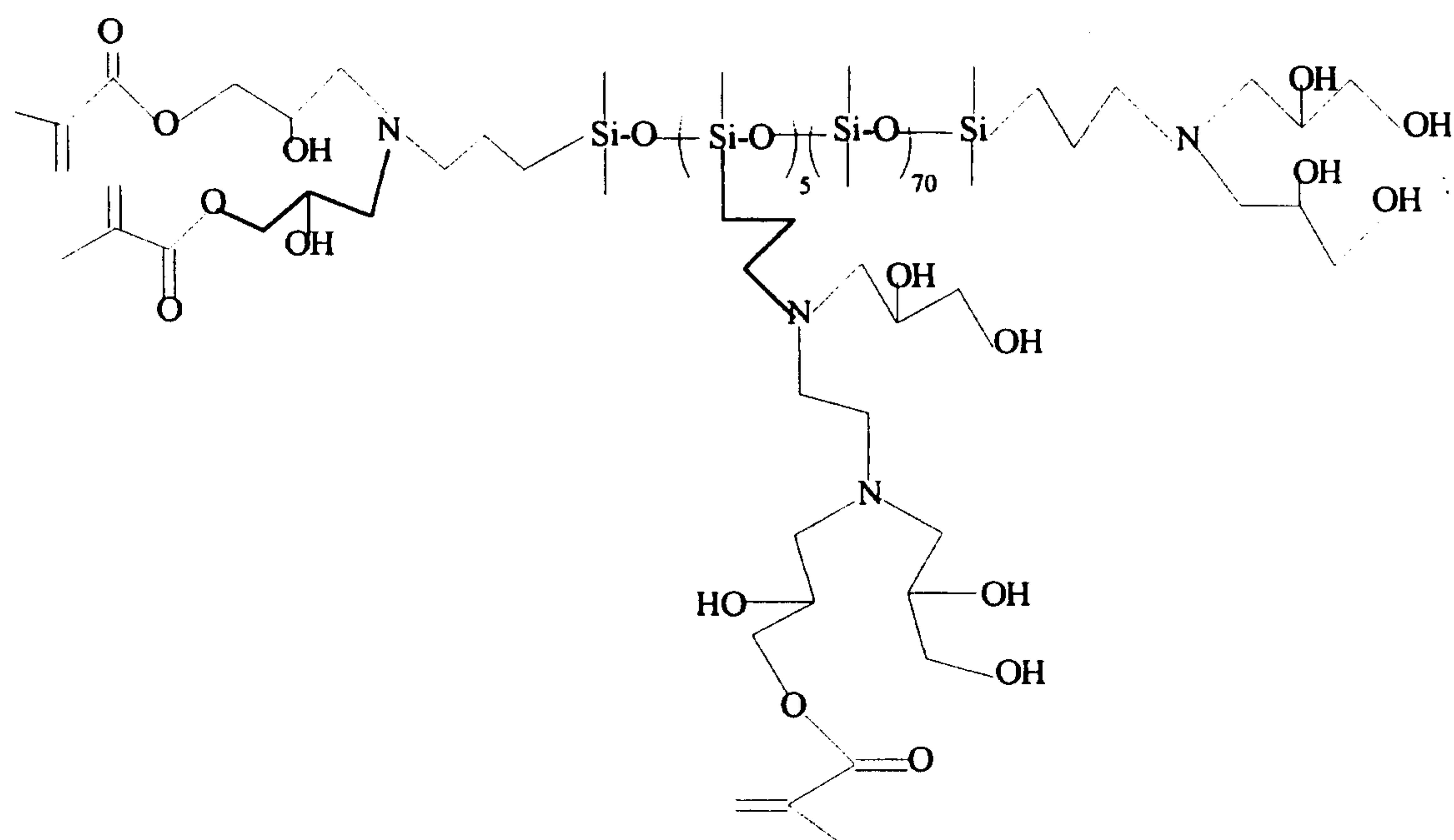
Structure VI,
