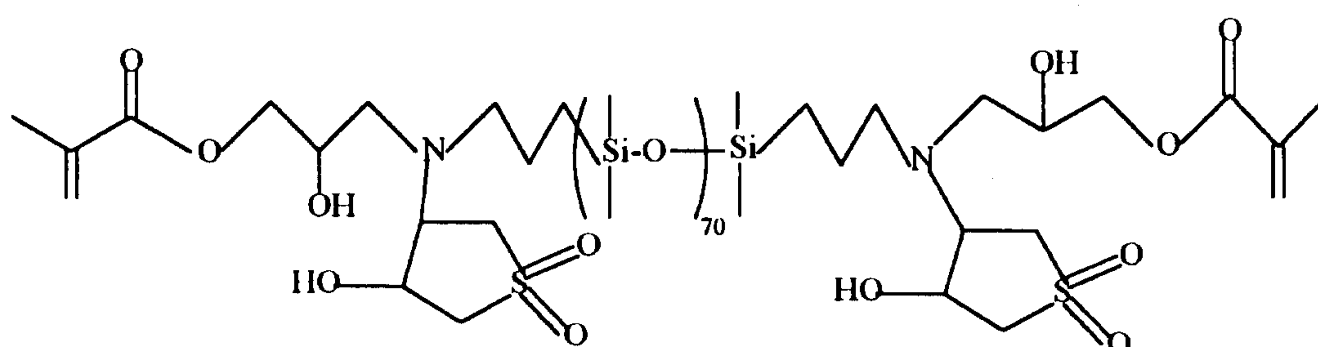
Structure XII,
