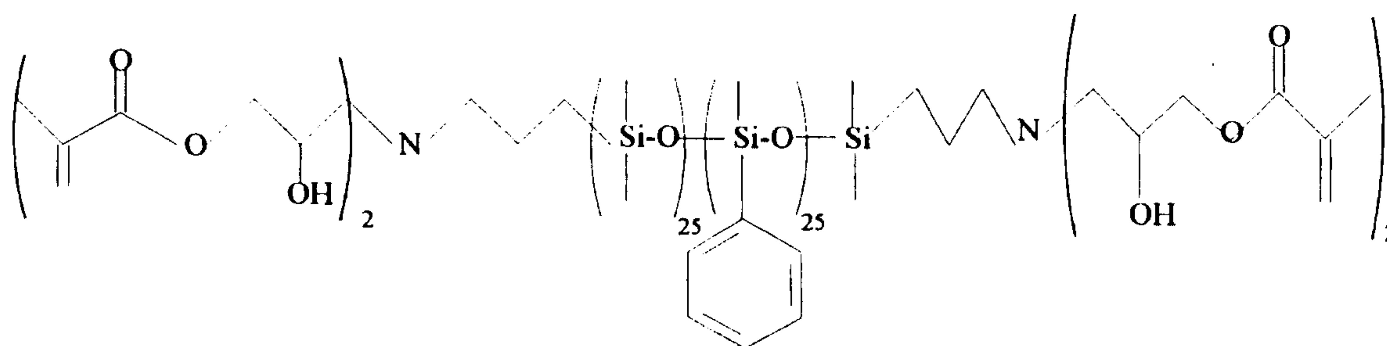
Structure X,
