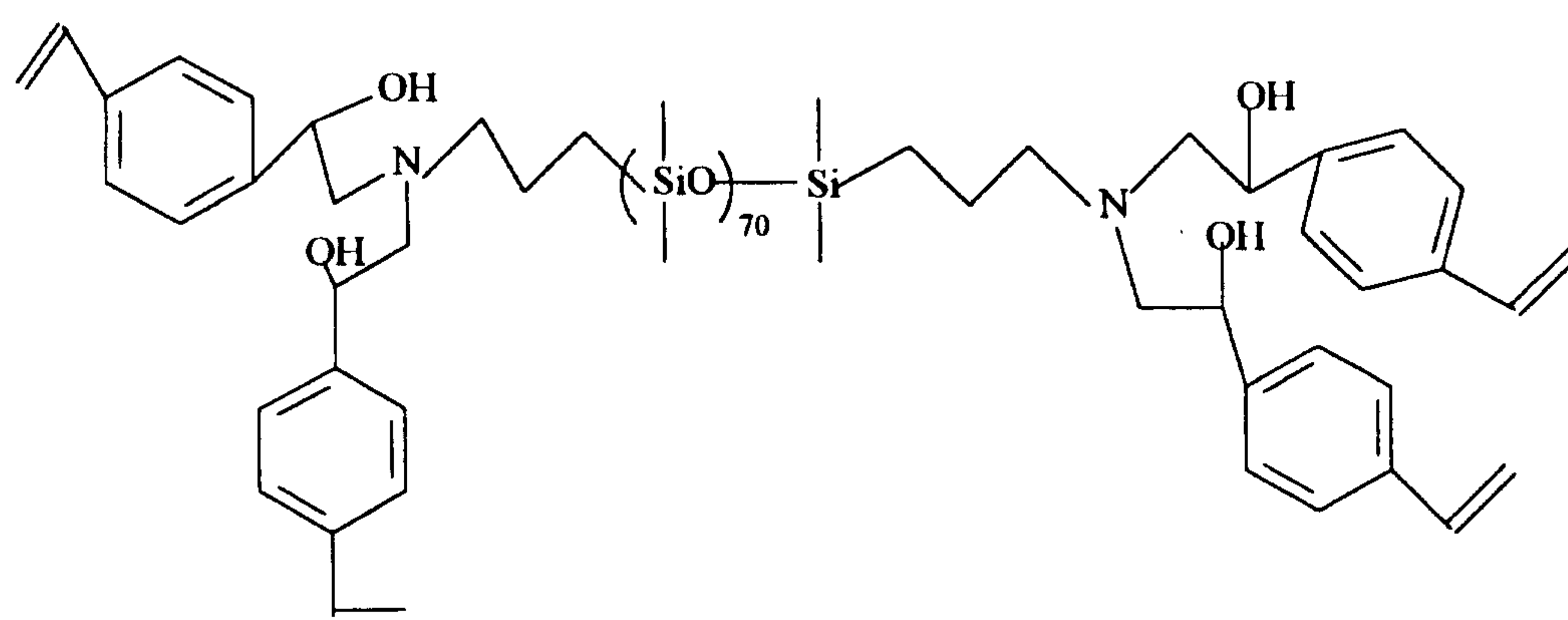
Structure VII,
