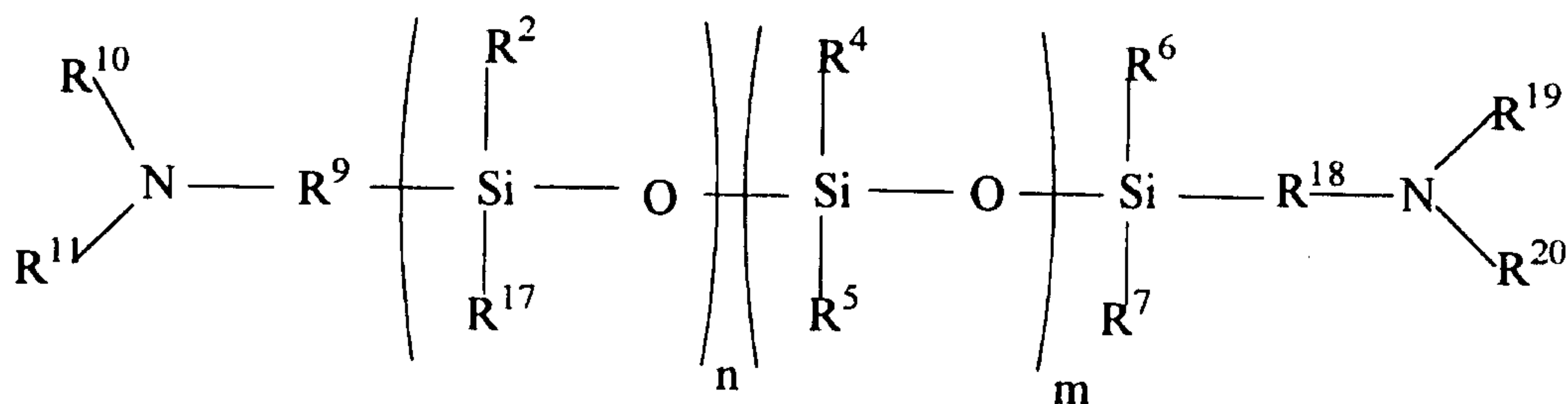
Structure IV
