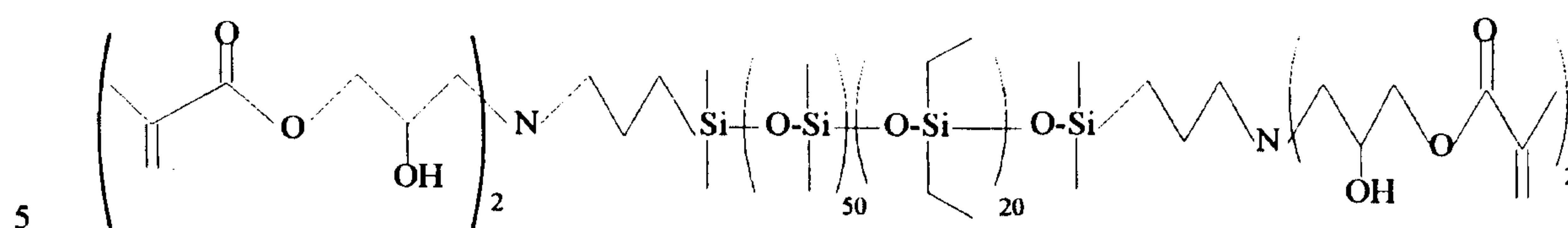
Structure XI,
