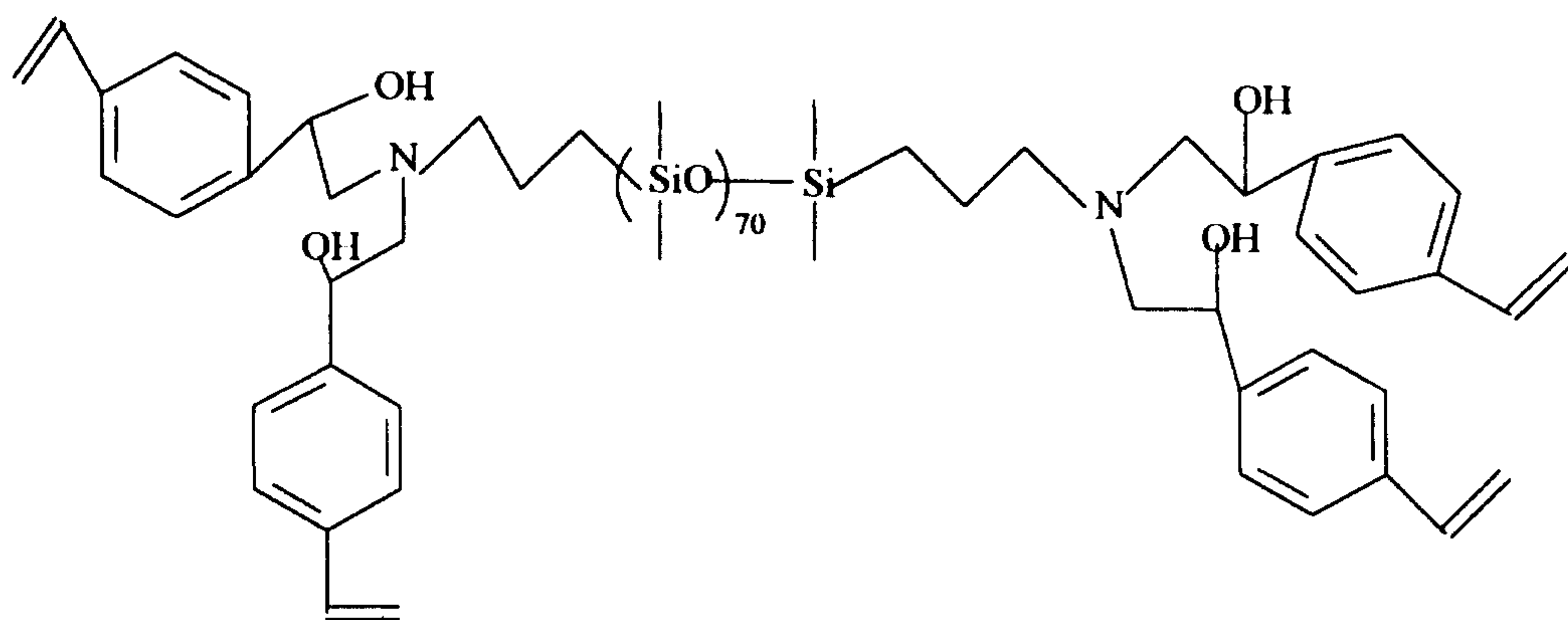
Structure VII,
