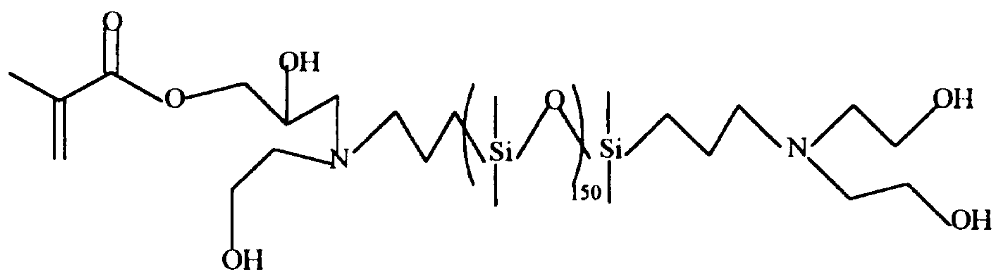
Structure VIII,
