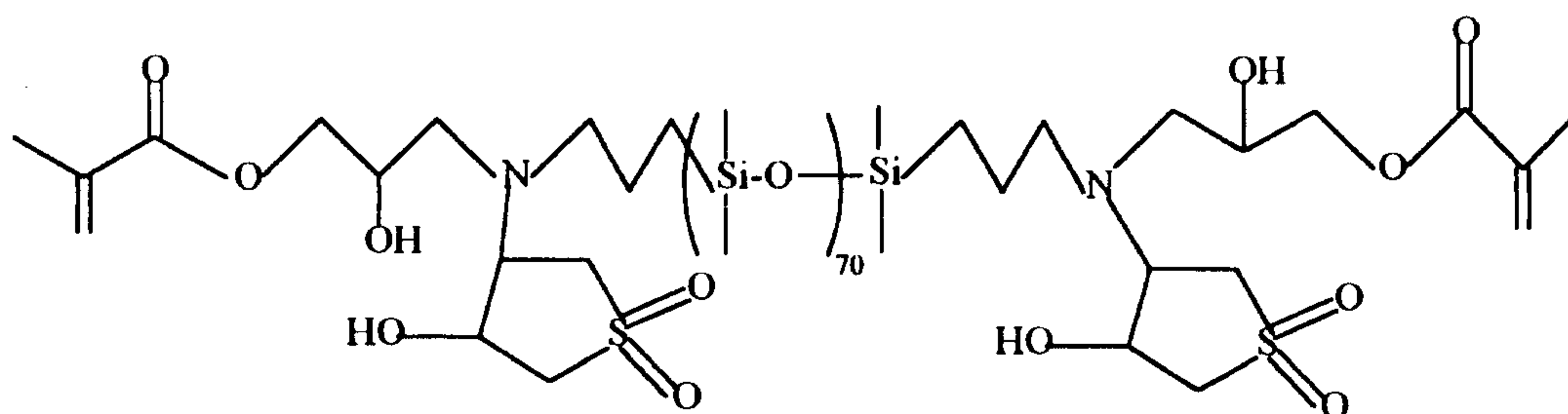
Structure XII,
