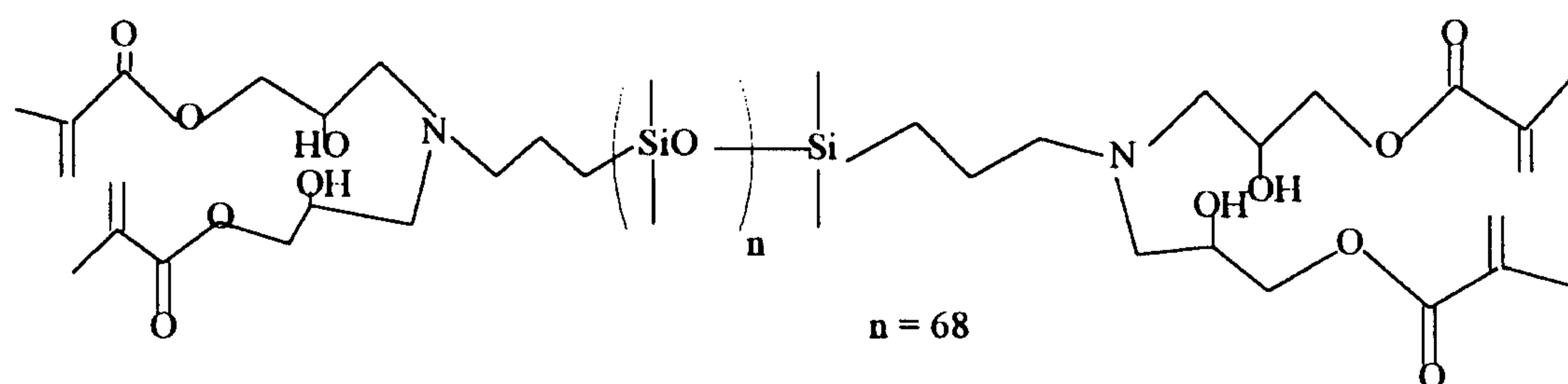
Structure V,
