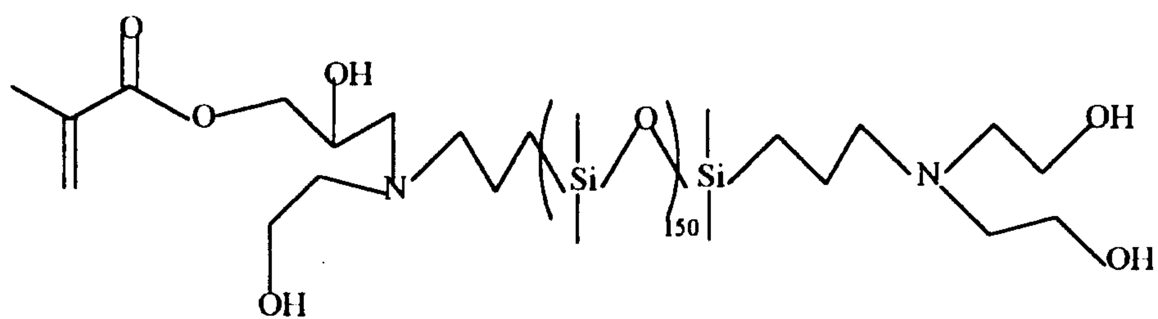
Structure VIII,
