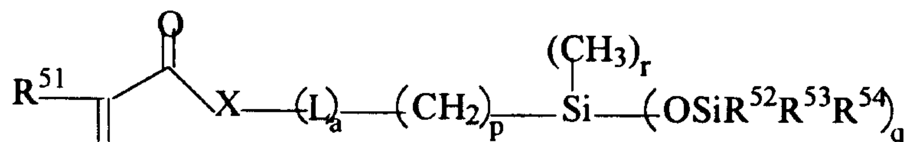
Structure XV
