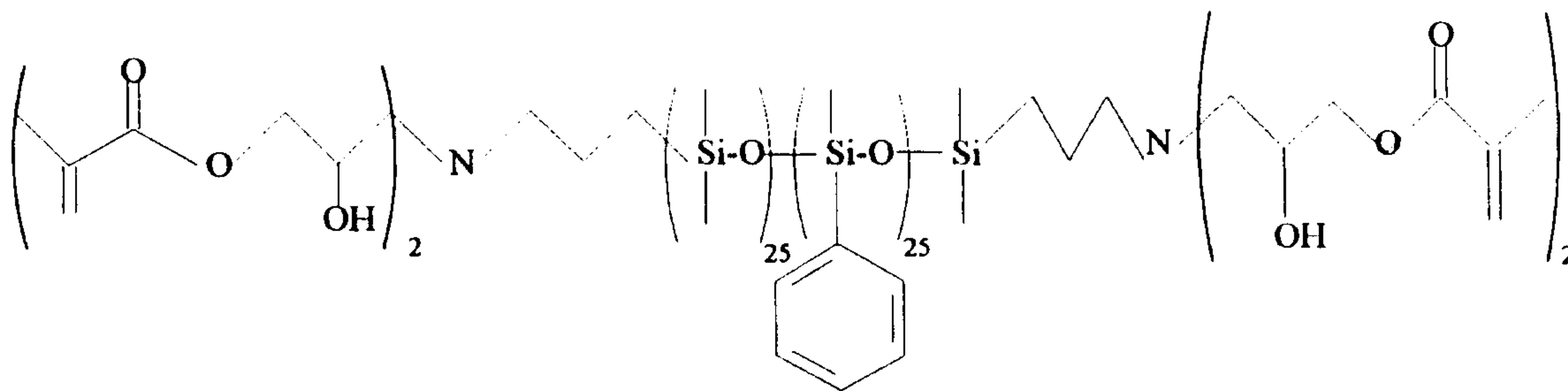
Structure X,
