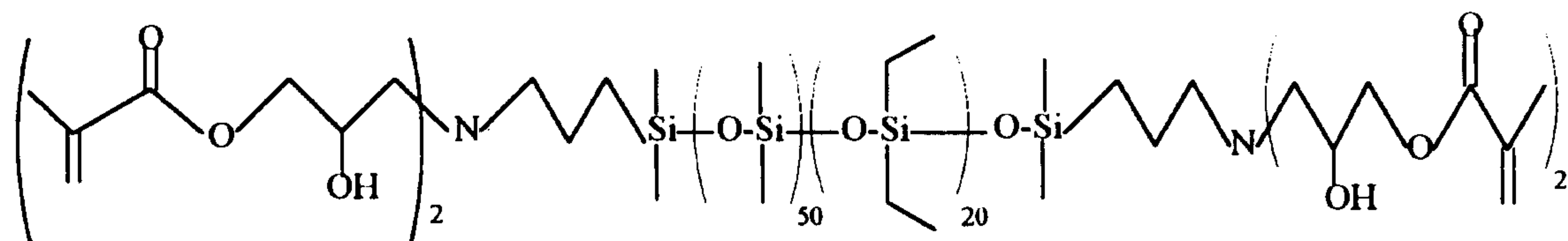
Structure XI,
