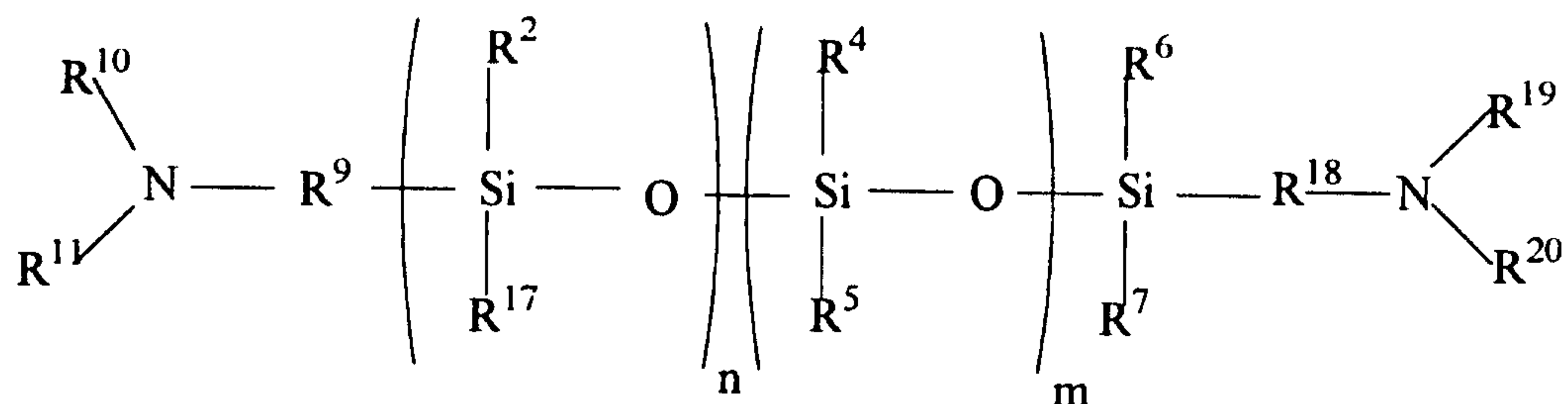
Structure IV
