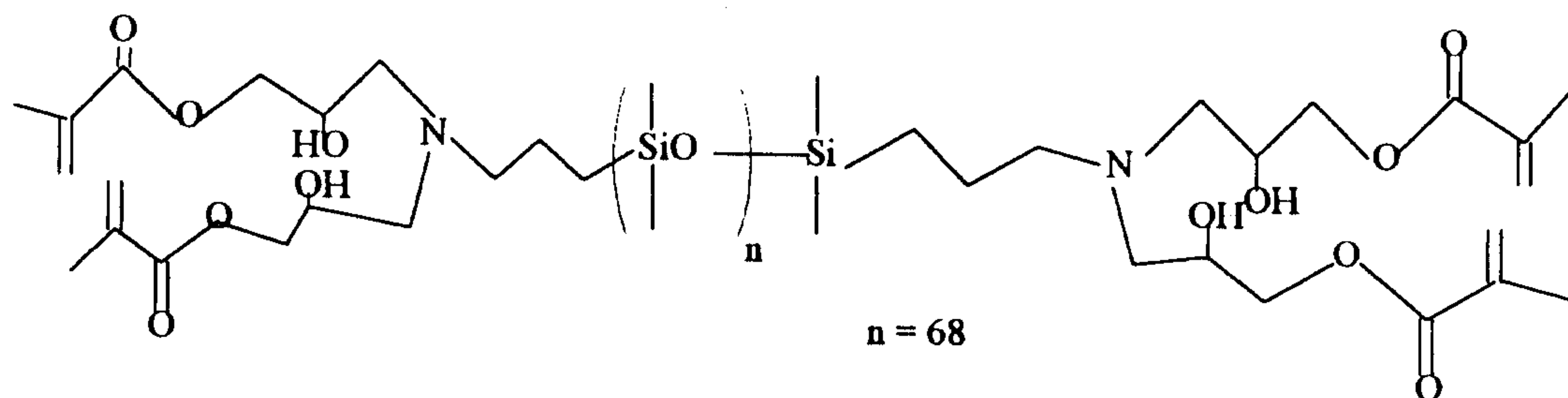
10 Structure V,
