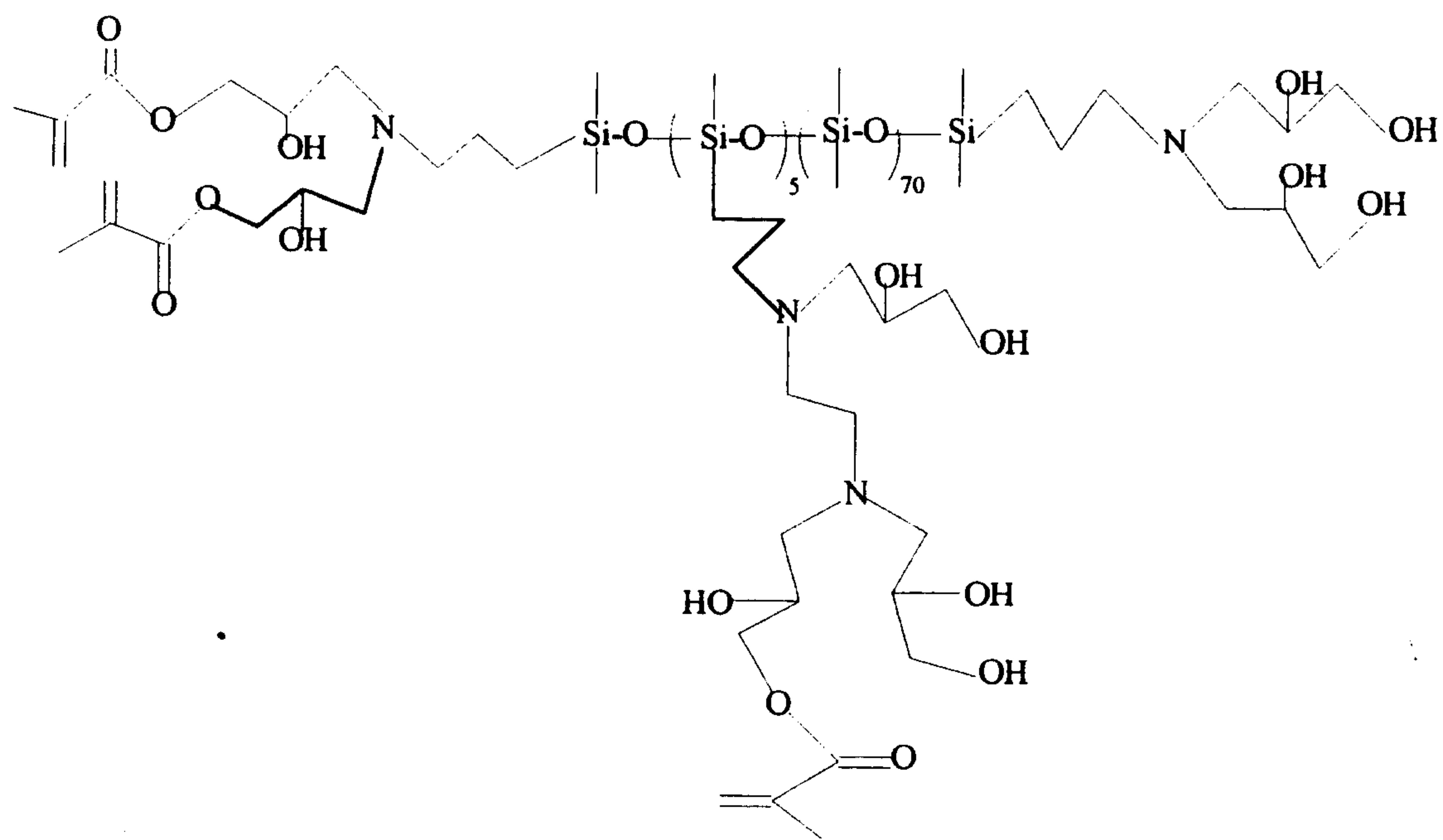
Structure VI,
