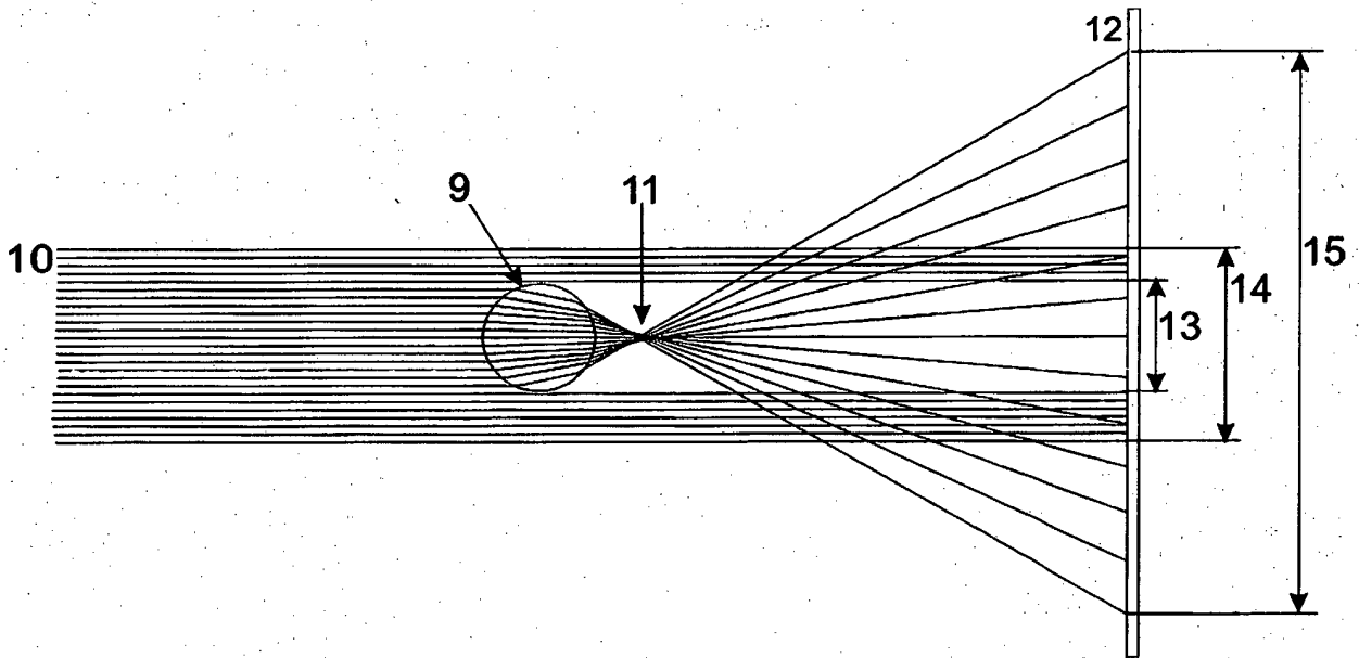
Figure 2 (Prior Art)
