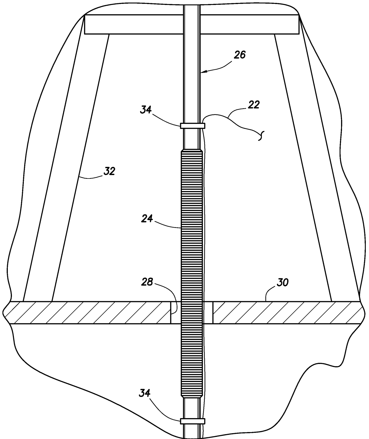
FIG. 2 (PRIOR ART)
