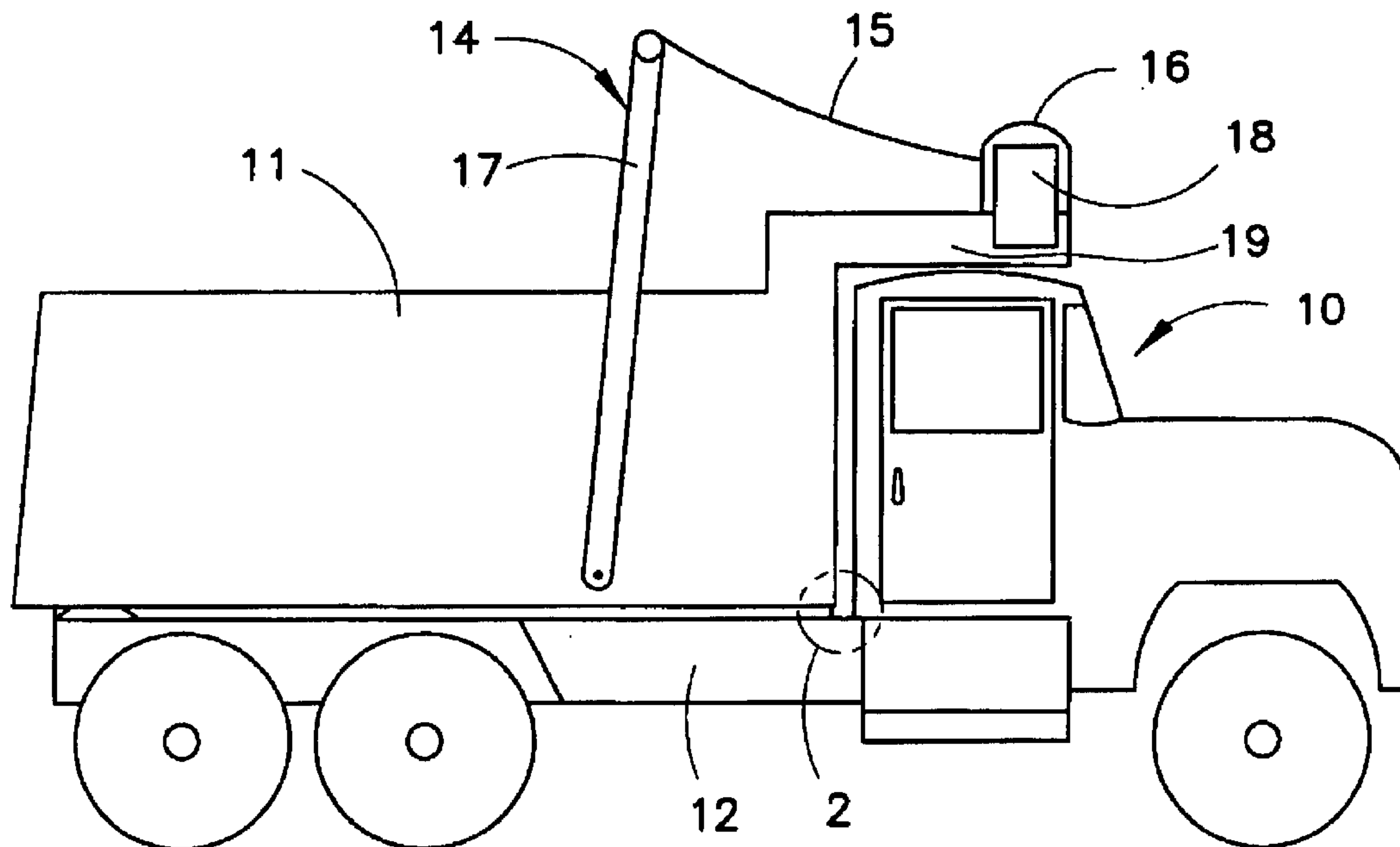
FIG. 1 (PRIOR ART)
