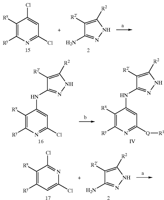
Scheme V
