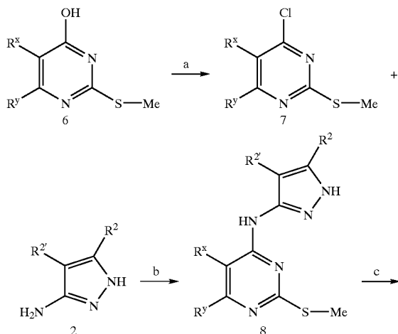
Scheme III
