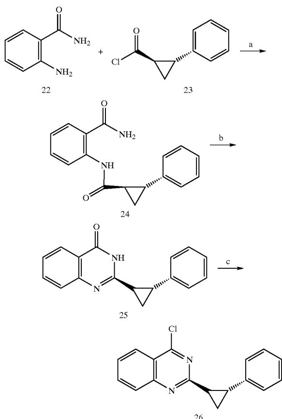
Scheme VII
