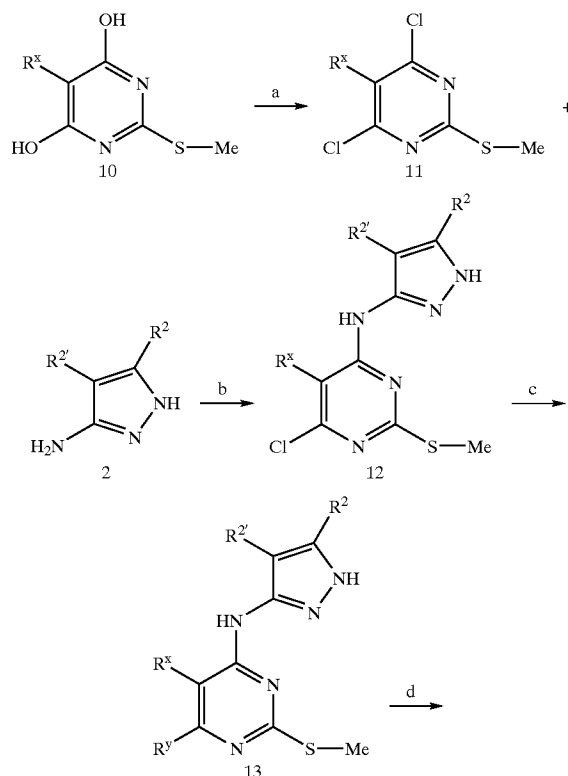
Scheme IV
