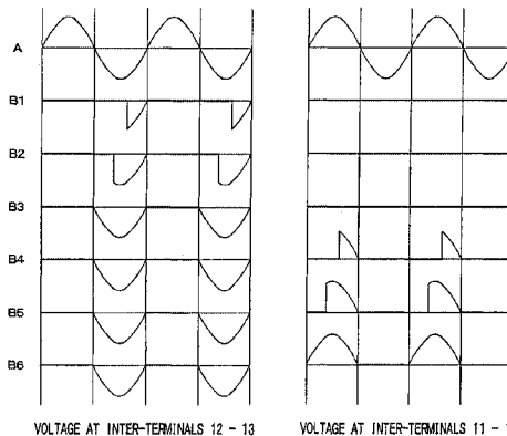
VOLTAGE AT INTER-TERMINALS 12 - 13
