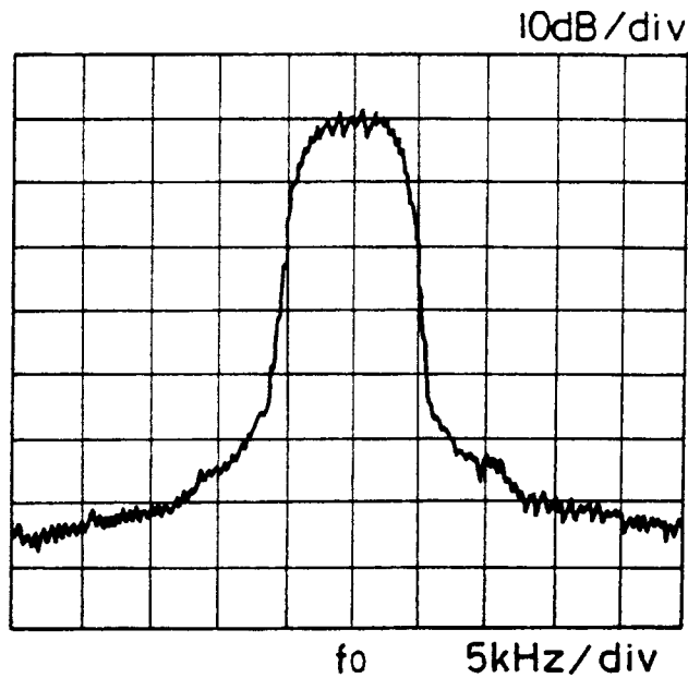
output characteristic ( signal converted )
