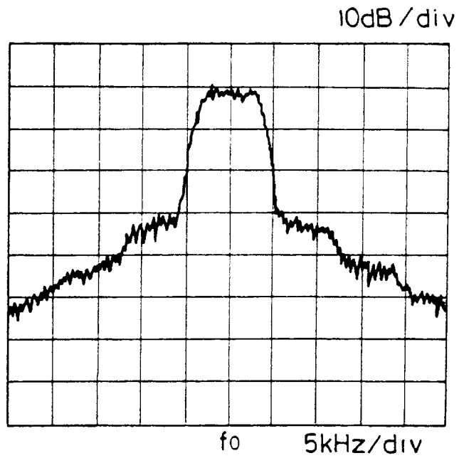
output characteristic ( no signal conversion )
