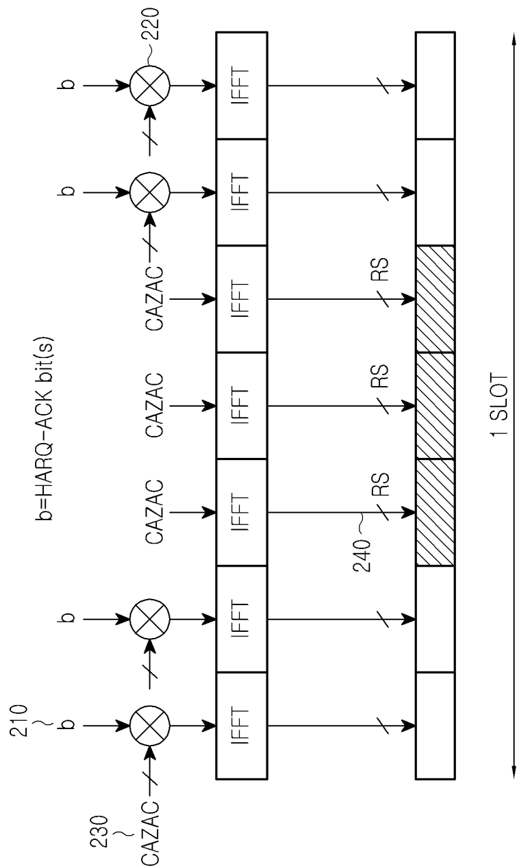
FIG. 2 (PRIOR ART)
