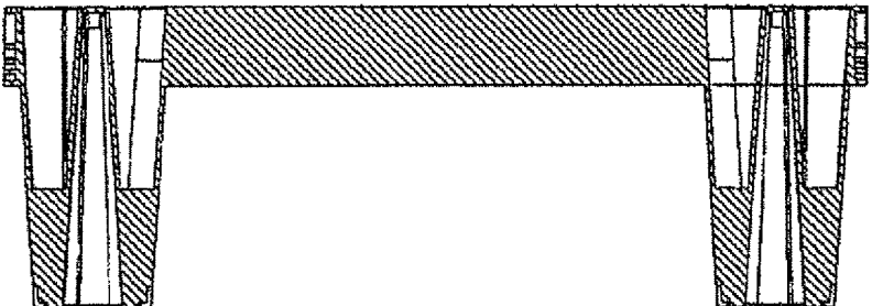
Fig. 82 Section C-C
