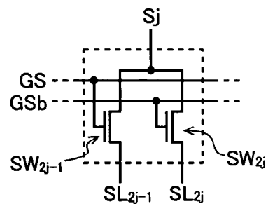
Fig. 2C PRIOR ART
