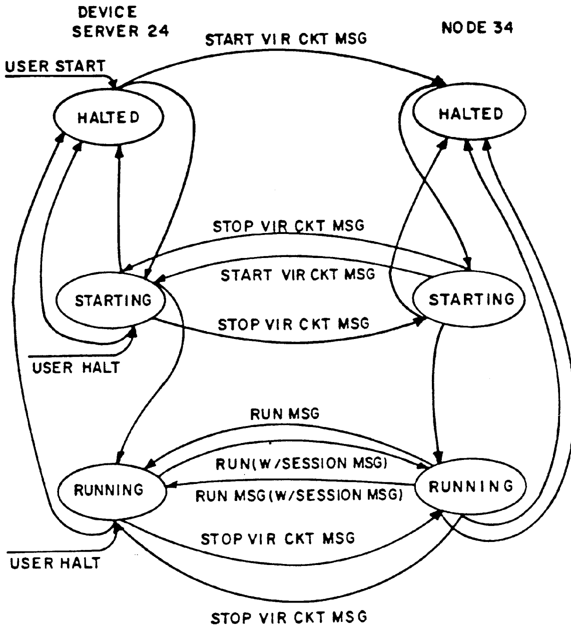
VIRTUAL CIRCUIT STATE DIAGRAM
