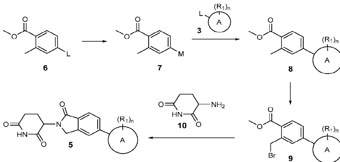
SCHEME 2
