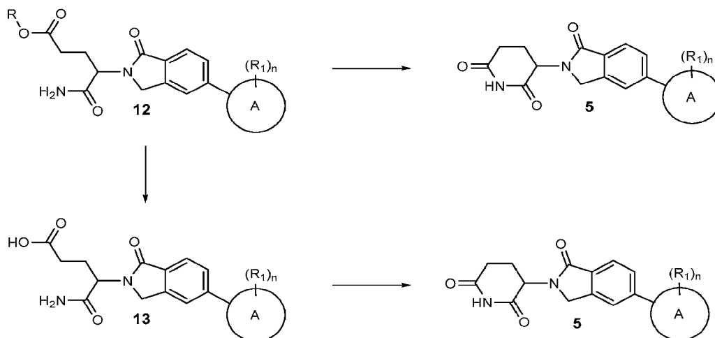
SCHEME 4
