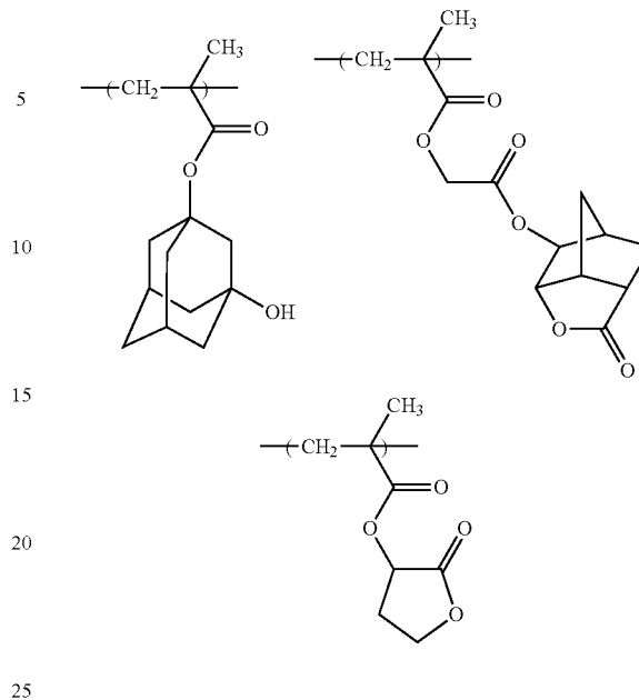
Synthetic Example 16
