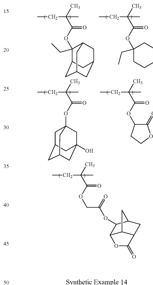
Synthetic Example 14
