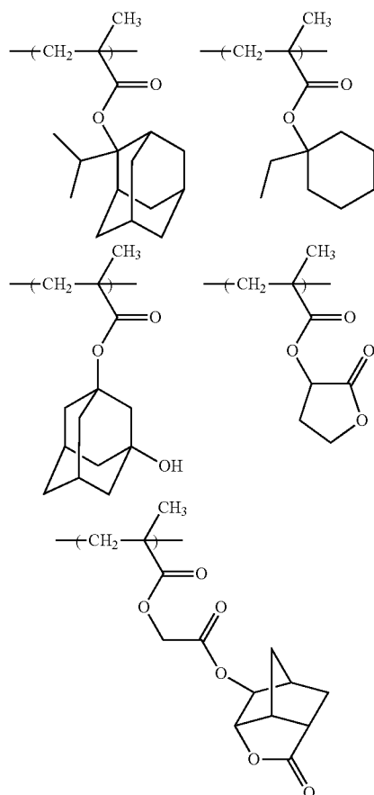
Synthetic Example 13
