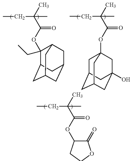
Synthetic Example 15
