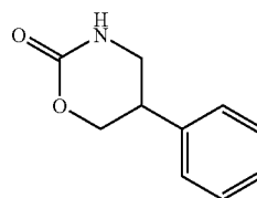
5-phenyl-1,3-oxazinan-2-one
