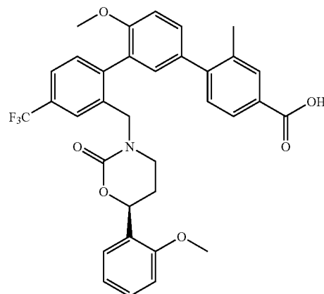
4'-methoxy-2''-{[(6S)-6-(2-methoxyphenyl)-2-oxo-1,3-oxazinan-3-yl]methyl}-2-methyl-4''-(trifluoromethyl)-1,1':3',1''-terphenyl-4-carboxylic acid
