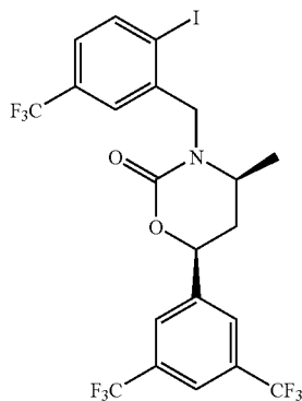
(4S,6S)-6-[3,5-bis(trifluoromethyl)phenyl]-3-[2-iodo-5-(trifluoromethyl)benzyl]-4-methyl-1,3-oxazinan-2-one
