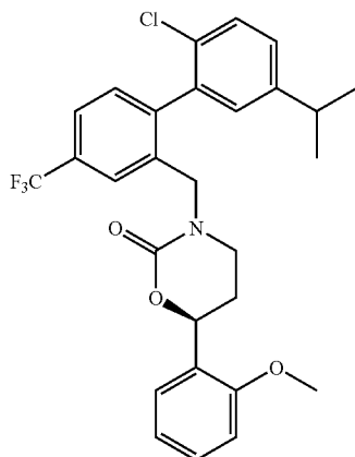
(6S)-3-([2'-chloro-5'-isopropyl-4-(trifluoromethyl)biphenyl-2-yl]methyl)-6-(2-methoxyphenyl)-1,3-oxazinan-2-one
