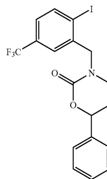
3-[2-iodo-5-(trifluoromethyl)benzyl]-6-phenyl-1,3-oxazinan-2-one
