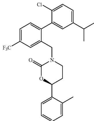
(6S)-3-([2'-chloro-5'-isopropyl-4-(trifluoromethyl)biphenyl-2-yl]methyl)-6-(2-methylphenyl)-1,3-oxazinan-2-one
