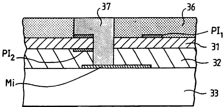
SECTION ON BB
