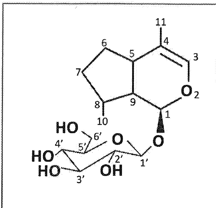
Iridoid
