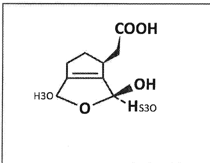
Non-Glycosidic Iridoid
