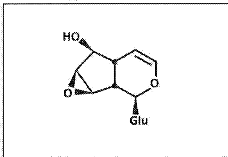
Glycosidic Iridoid
