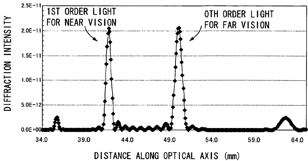
DIFFRACTION INTENSITY ALONG OPTICAL AXIS (COMPARATIVE EXAMPLE 1)
