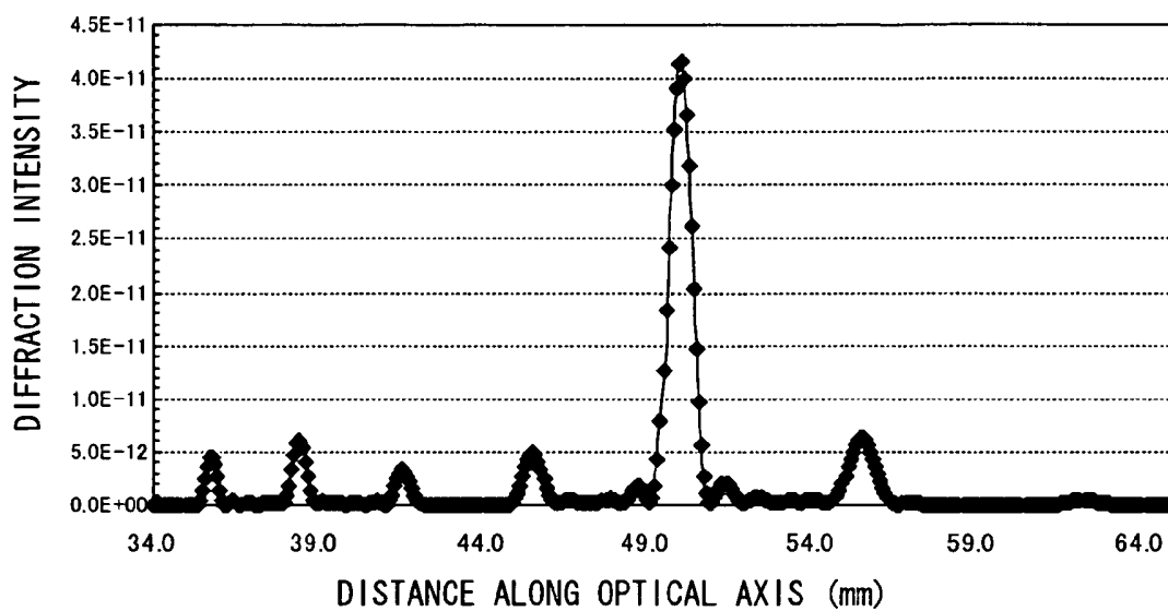
DIFFRACTION INTENSITY ALONG OPTICAL AXIS (COMPARATIVE EXAMPLE 2)
