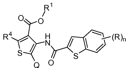
; Formula (X)
