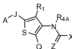
Formula (VII);
