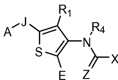
Formula (VIII);
