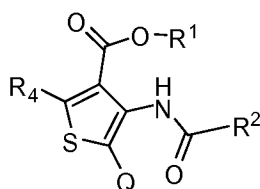
Formula (IX)
