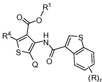
Formula (XA)
