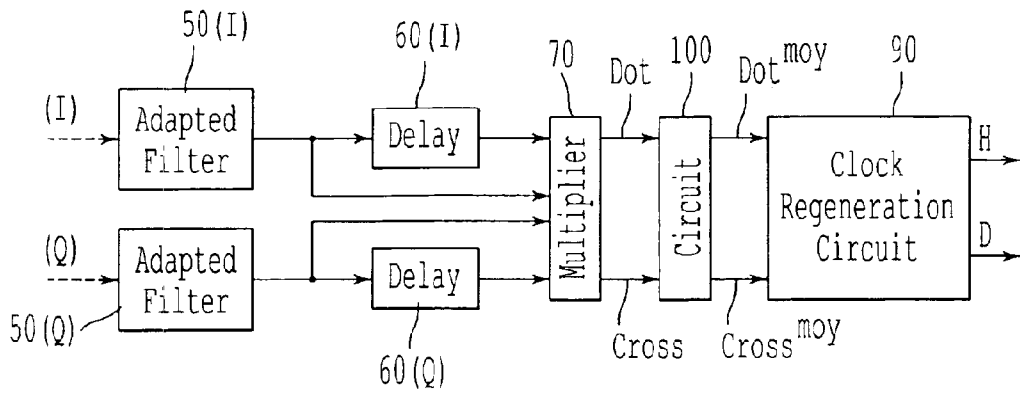
FIG. 4 BACKGROUND ART
