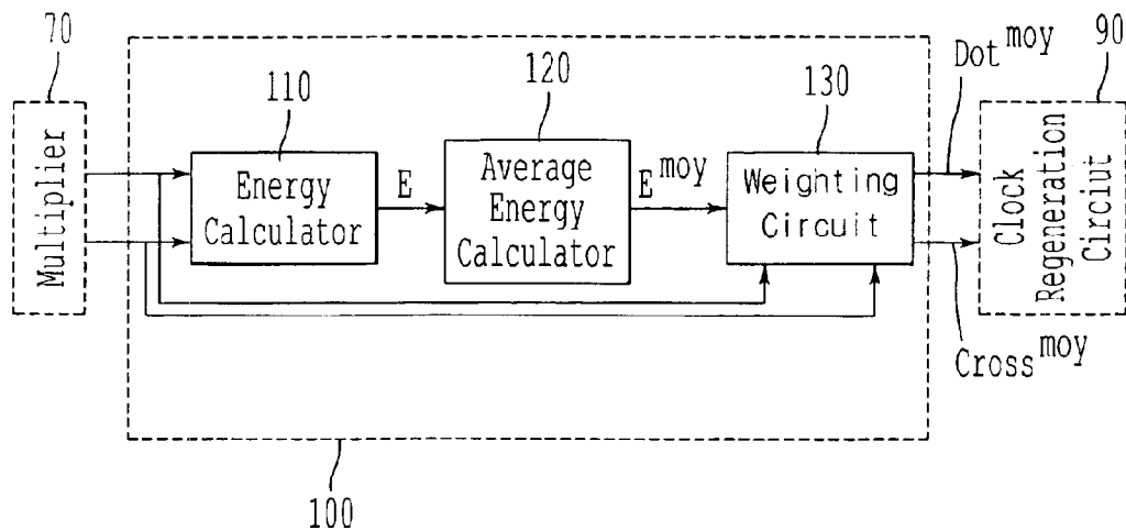
FIG. 5 BACKGROUND ART
