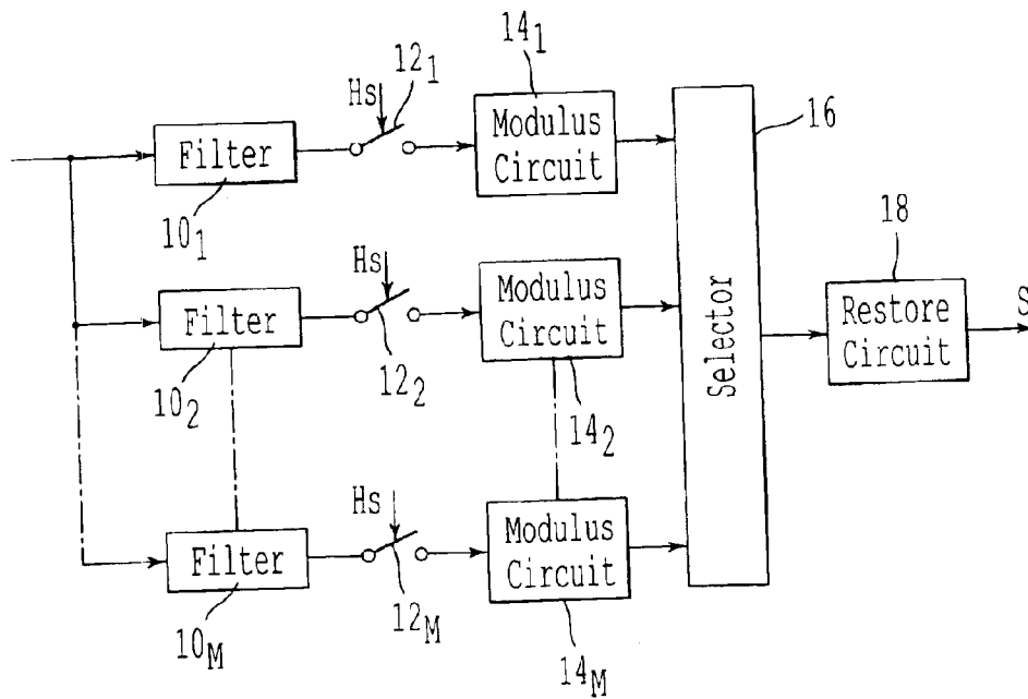
FIG. 1 BACKGROUND ART
