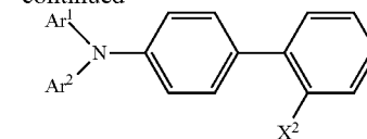
Compound B
