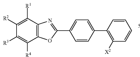
Compound A
