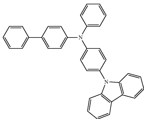
p-YGA1BP
