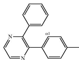
4-(3-phenylpyrazin-2-yl)phenyl
