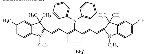
Infrared absorbent (2)
