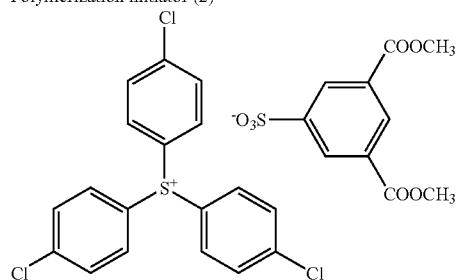
Polymerization initiator (2)
